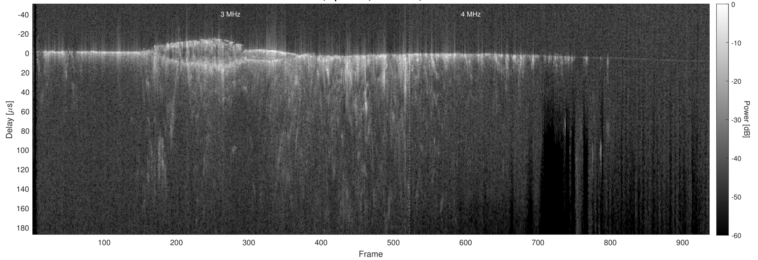
Orbit 13821, Optimized, No Window, Channel 2
