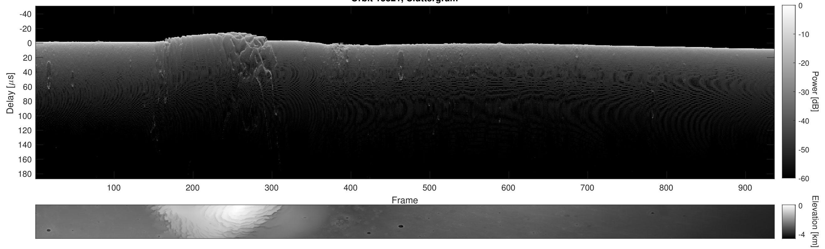
Orbit 13821, Cluttergram
