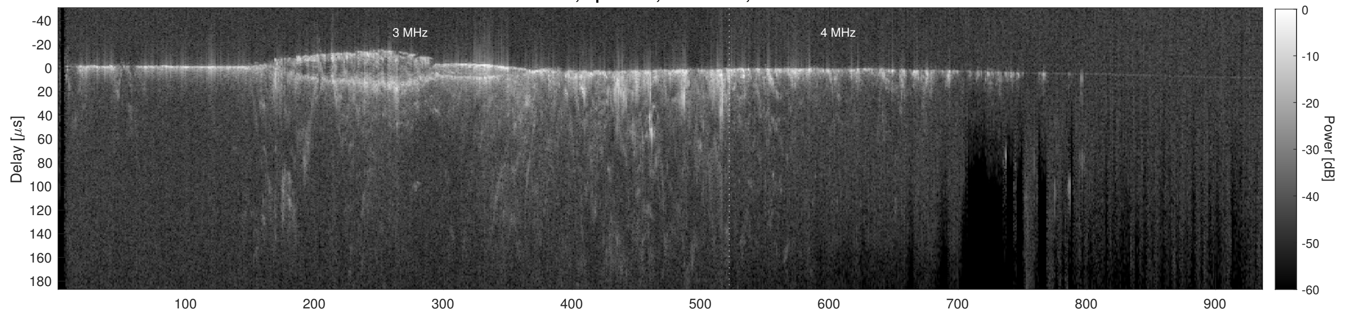
Orbit 13821, Cluttergram
