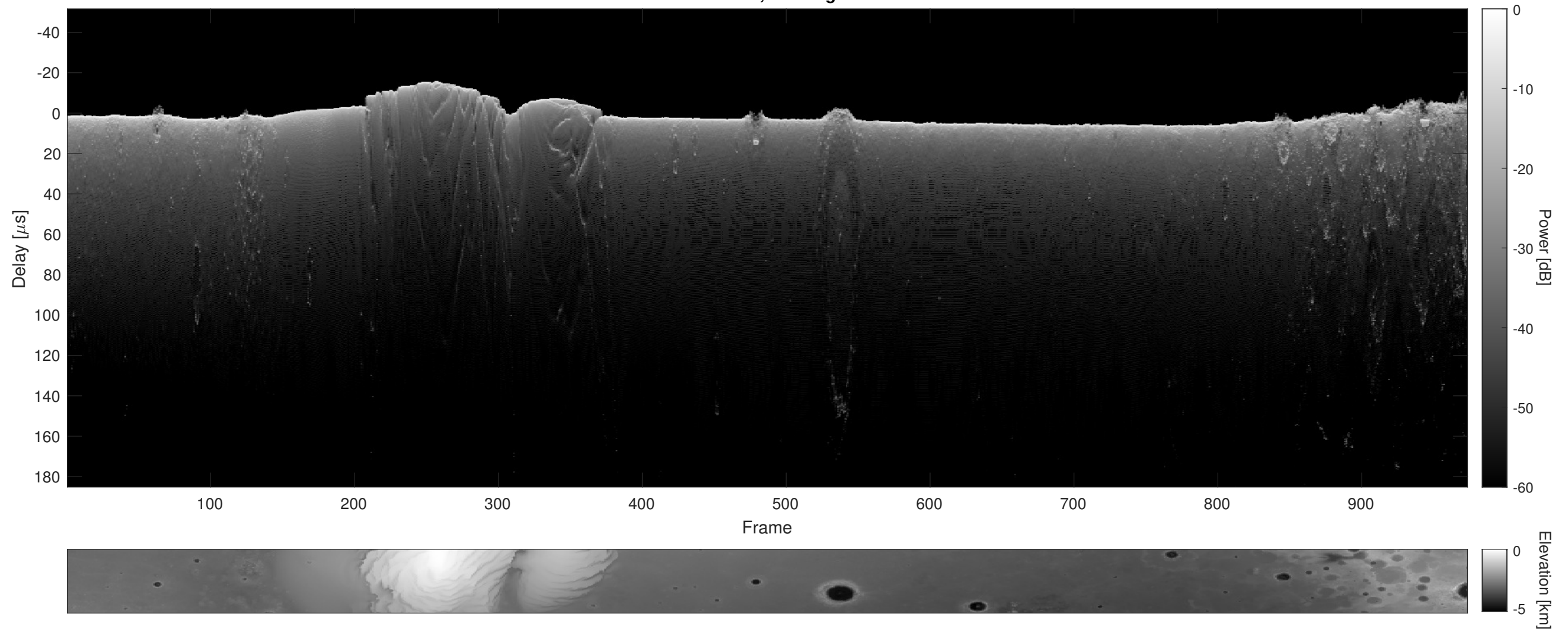
Orbit 13823, Cluttergram
