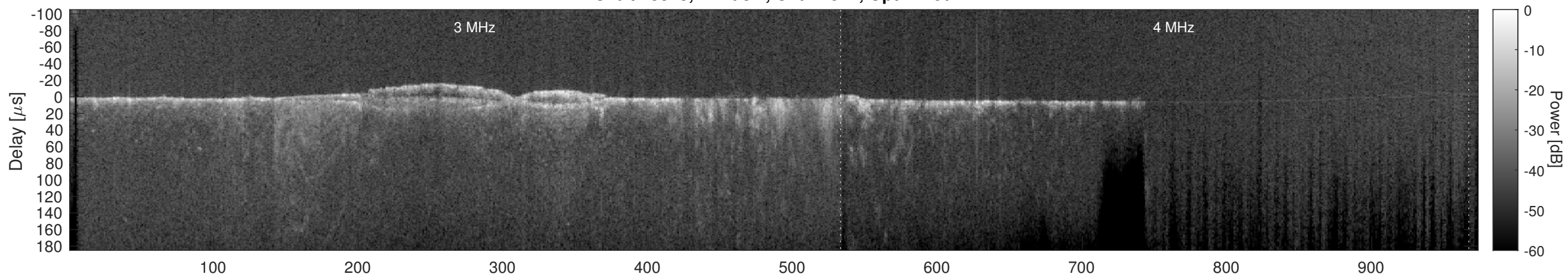
Orbit 13823, Cluttergram
