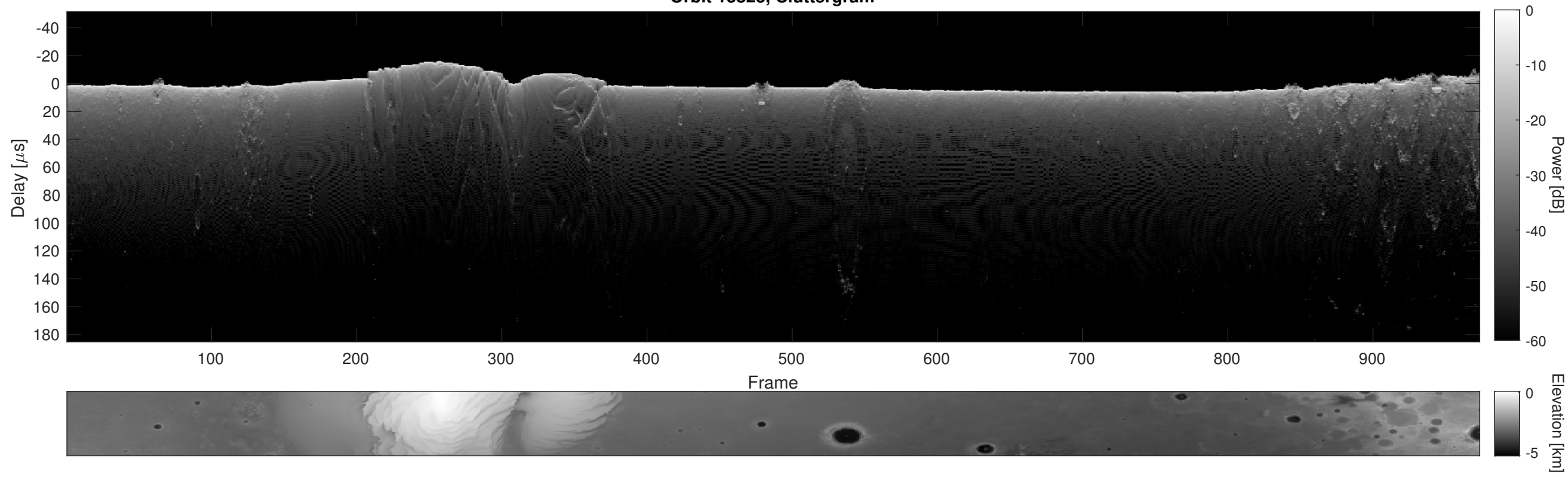
Orbit 13823, Cluttergram
