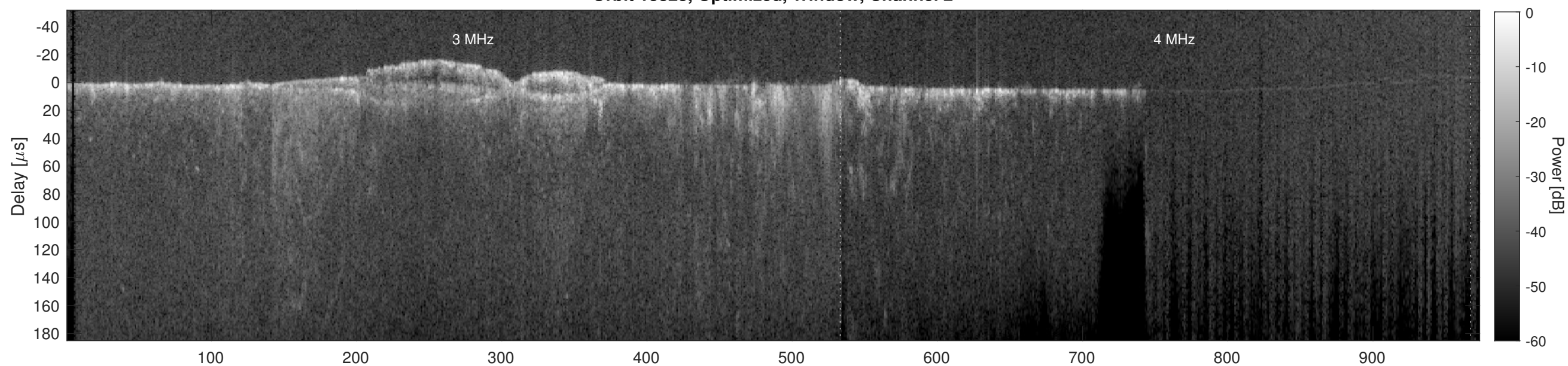
Orbit 13823, Cluttergram
