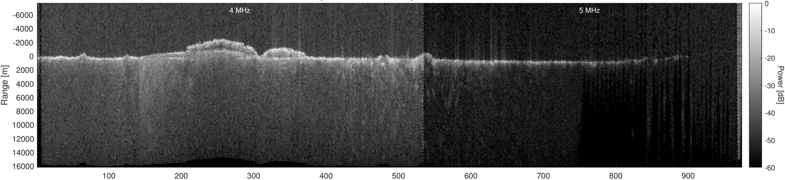
Orbit 13823, Optimized, Window, Depth-Corrected, Channel 2
