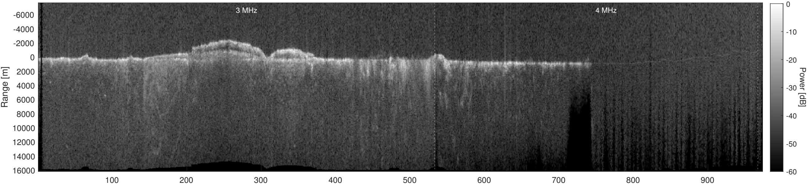
Orbit 13823, Depth-Corrected Cluttergram
