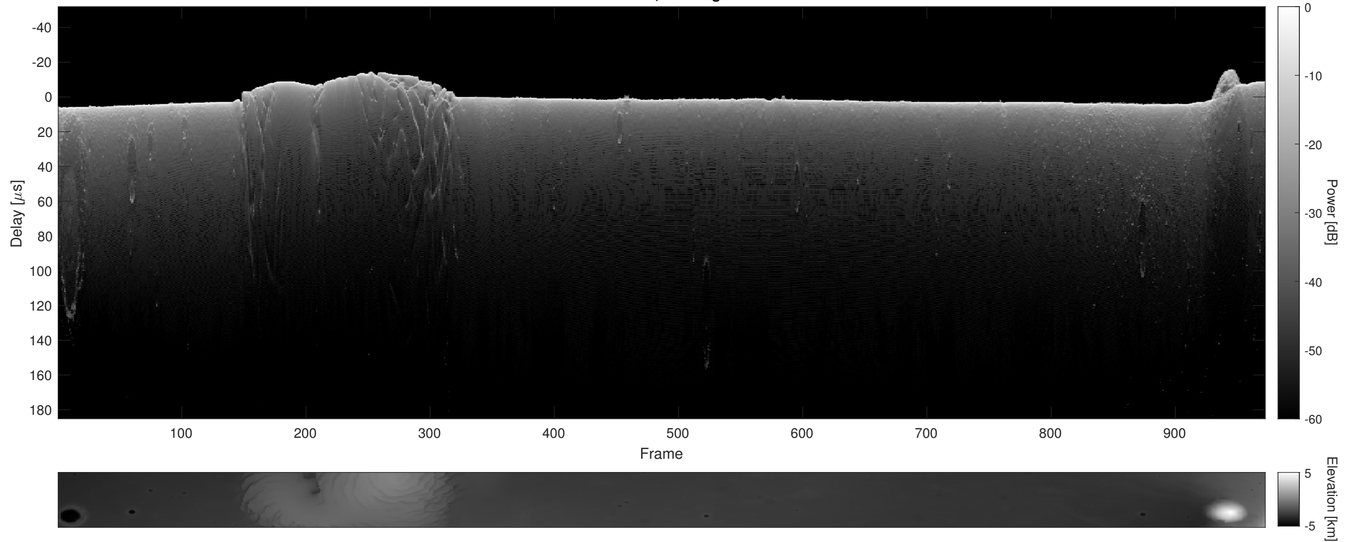
Orbit 13825, Cluttergram
