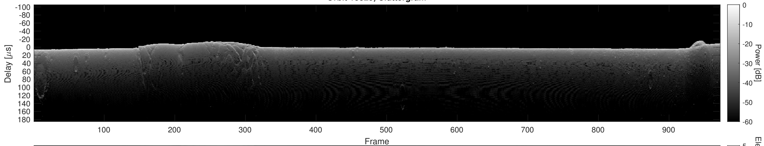
Orbit 13825, Cluttergram
