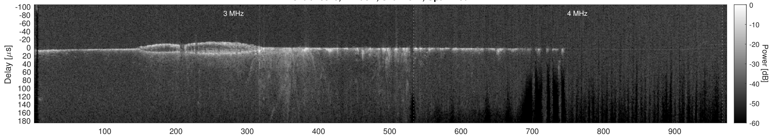
Orbit 13825, Cluttergram
