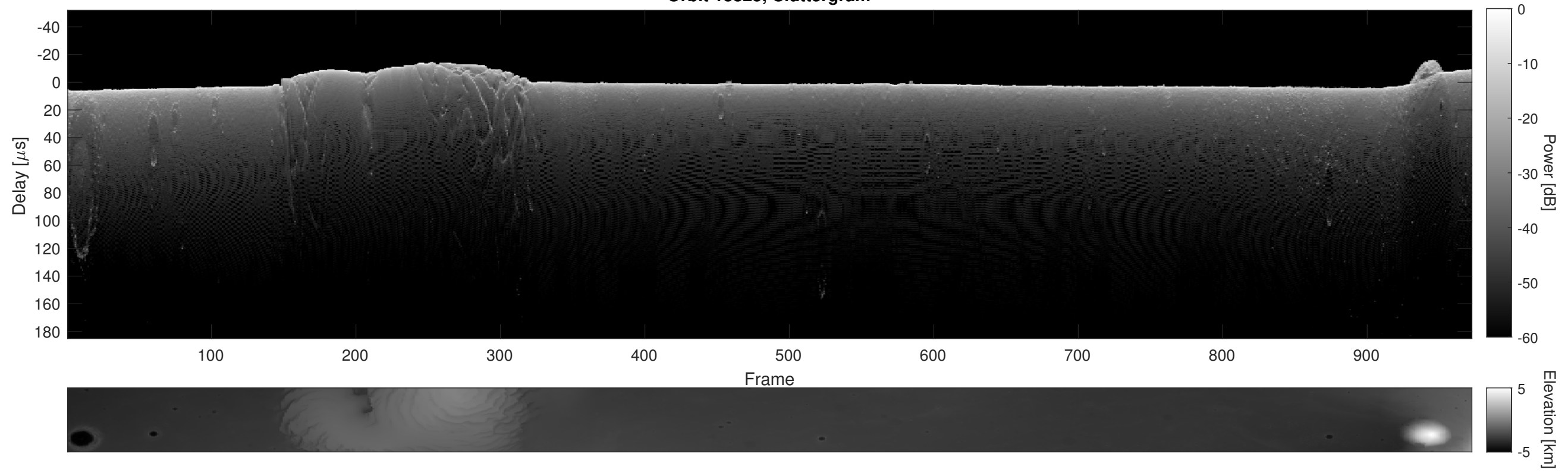
Orbit 13825, Cluttergram
