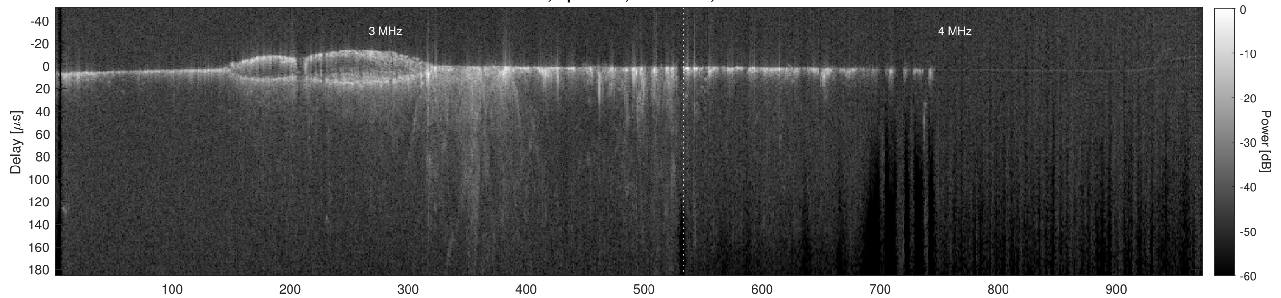
Orbit 13825, Cluttergram
