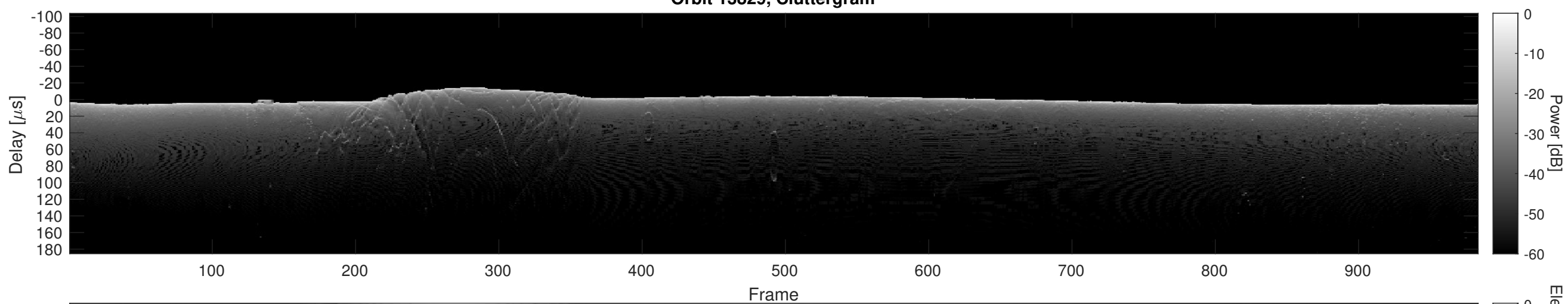
Orbit 13829, Cluttergram
