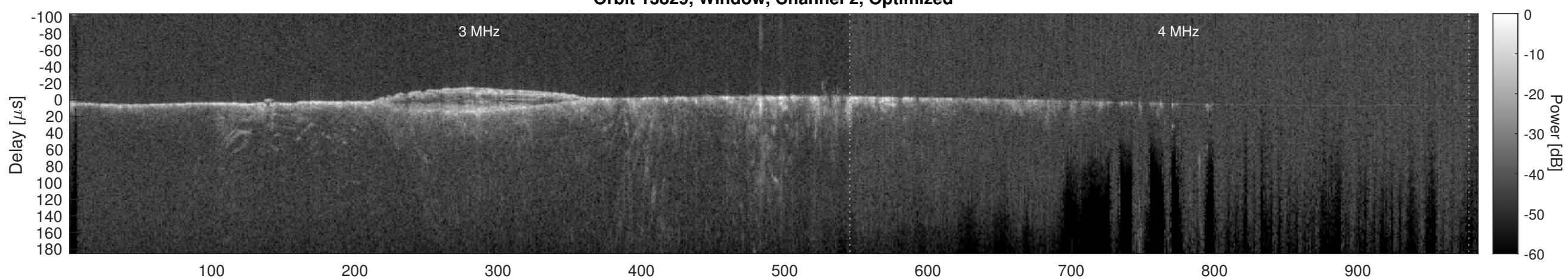
Orbit 13829, Cluttergram
