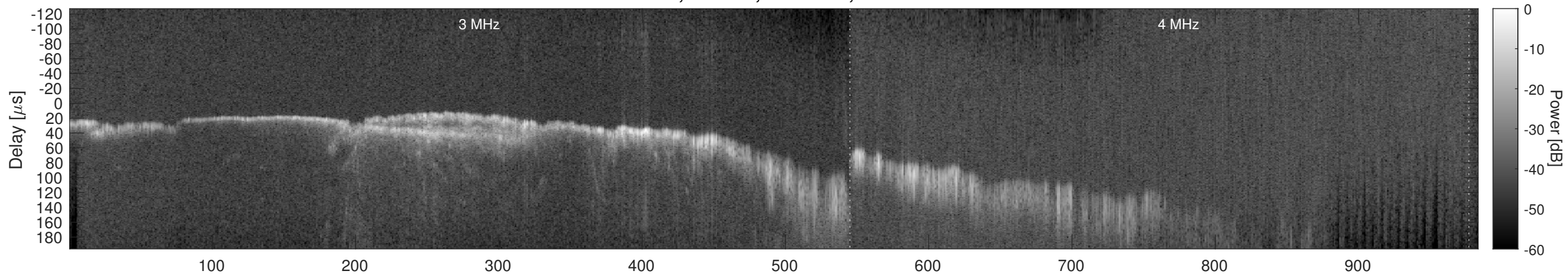
Orbit 13831, Window, Channel 2, Chapman
