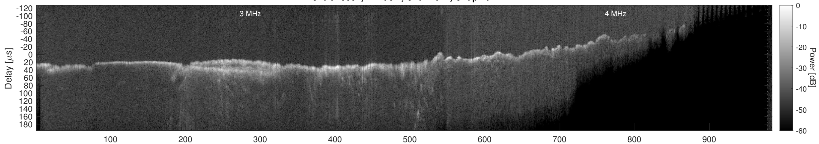
Orbit 13831, Window, Channel 2, Optimized
