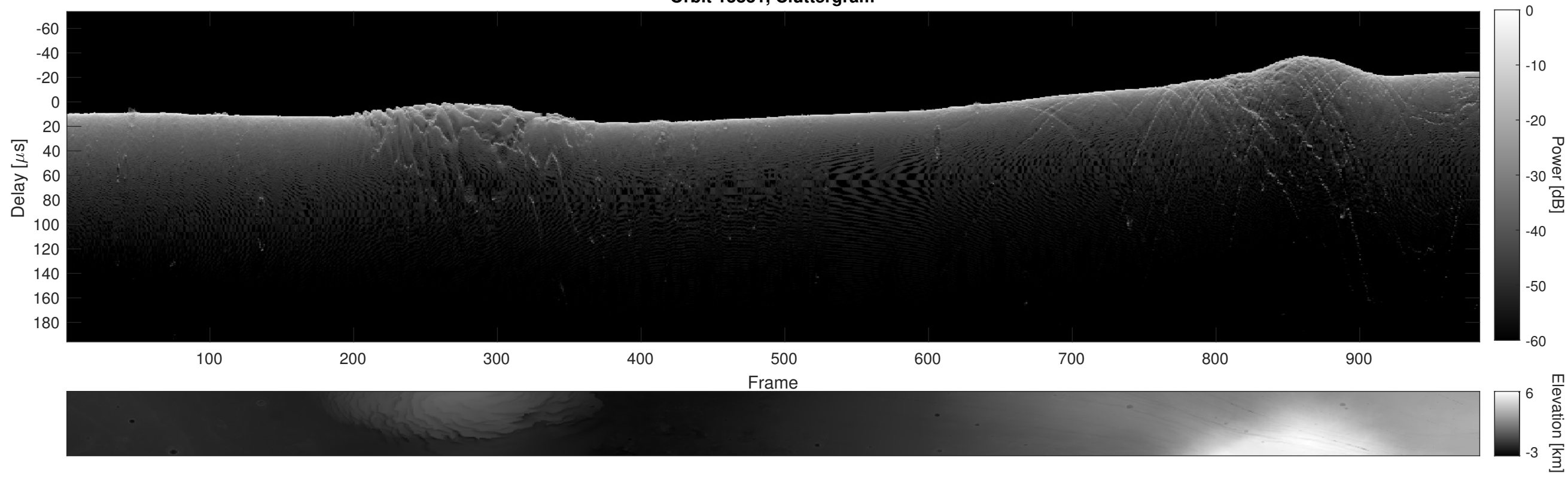
Orbit 13831, Cluttergram
