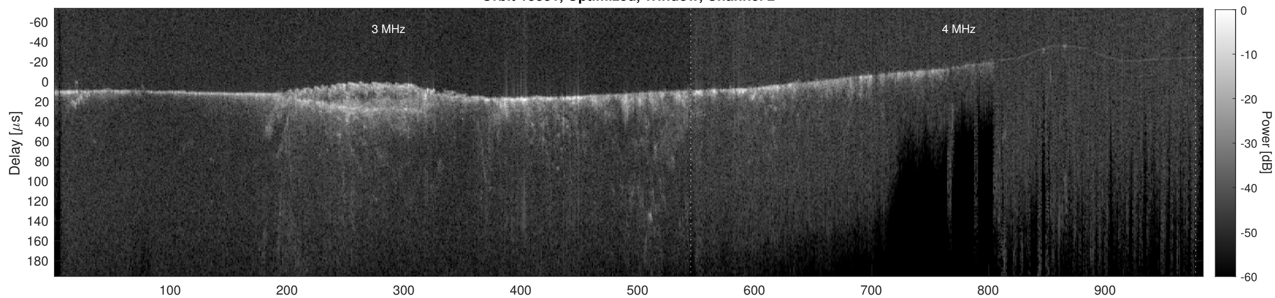
Orbit 13831, Cluttergram
