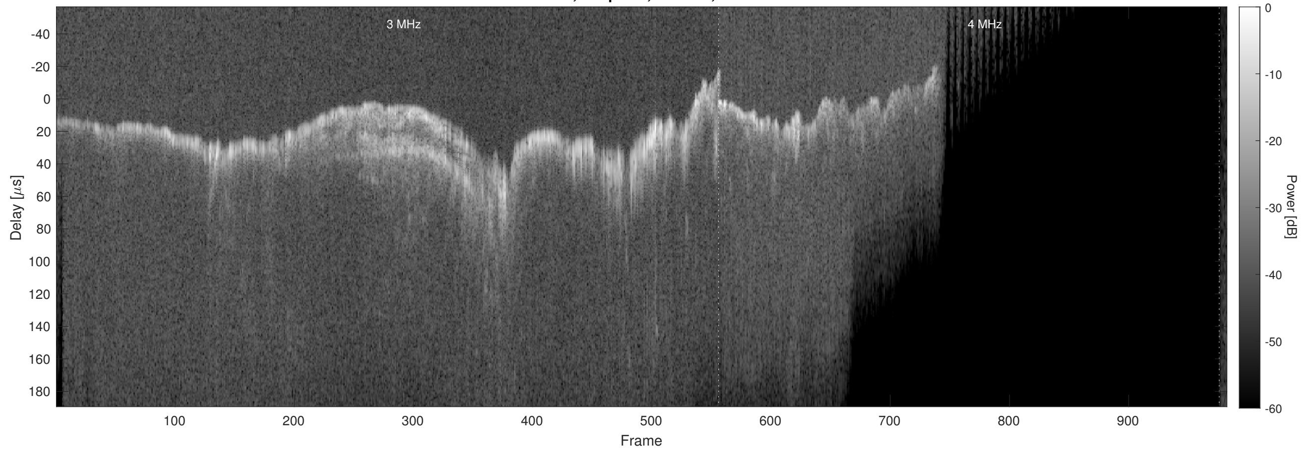
Orbit 13833, Chapman, Window, Channel 2
