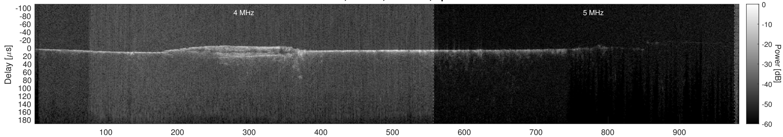
Orbit 13833, Cluttergram
