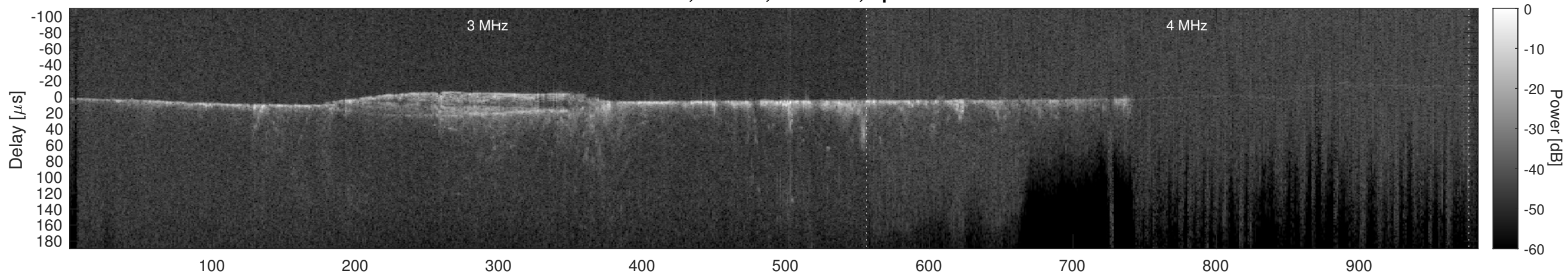
Orbit 13833, Cluttergram
