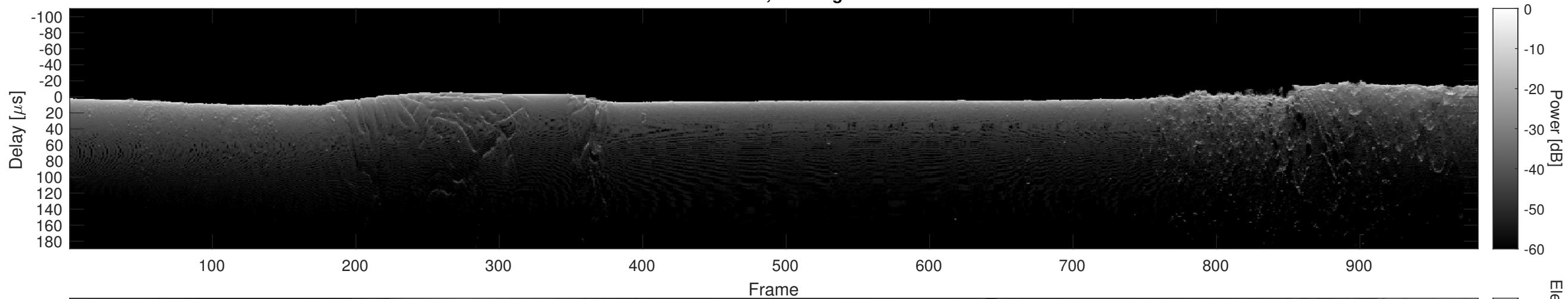
Orbit 13833, Cluttergram
