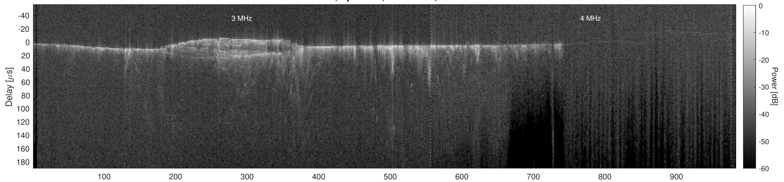
Orbit 13833, Cluttergram
