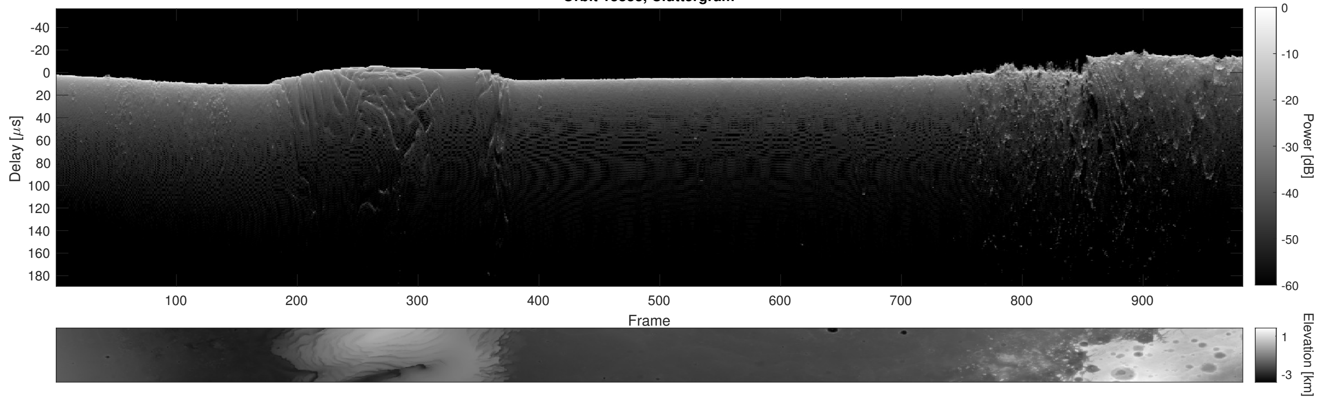
Orbit 13833, Cluttergram
