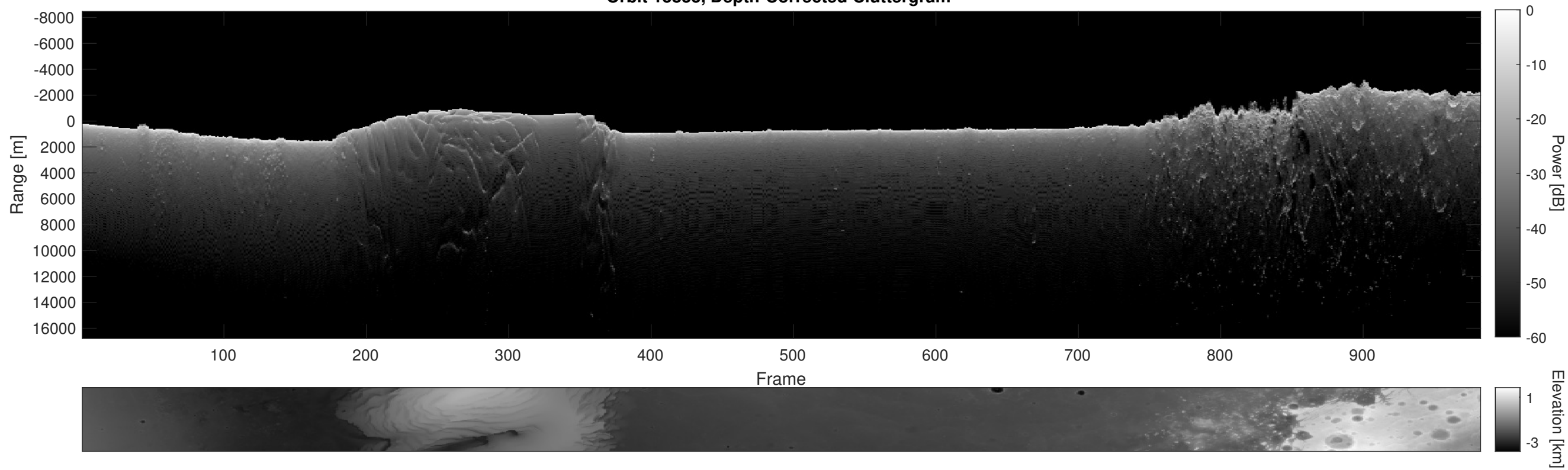
Orbit 13833, Depth-Corrected Cluttergram
