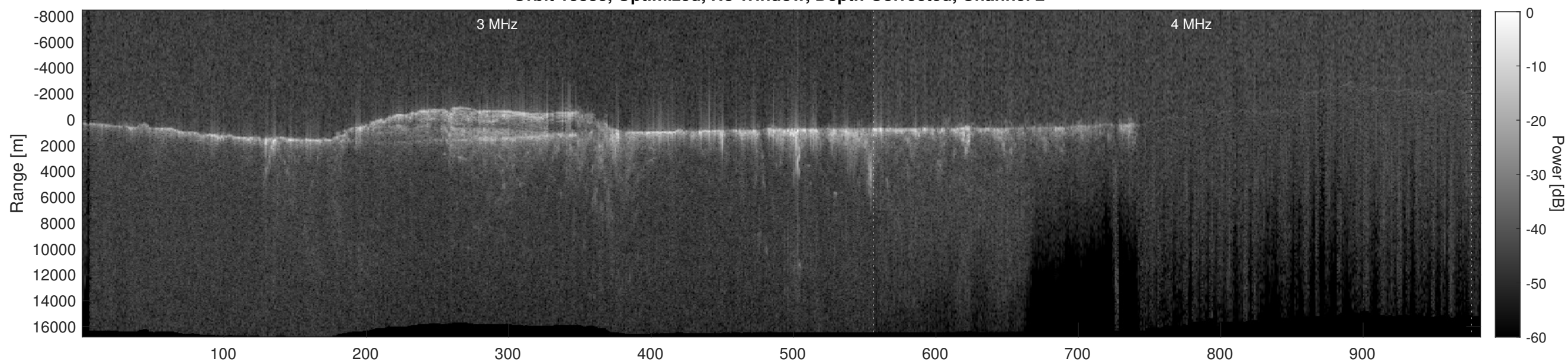
Orbit 13833, Depth-Corrected Cluttergram
