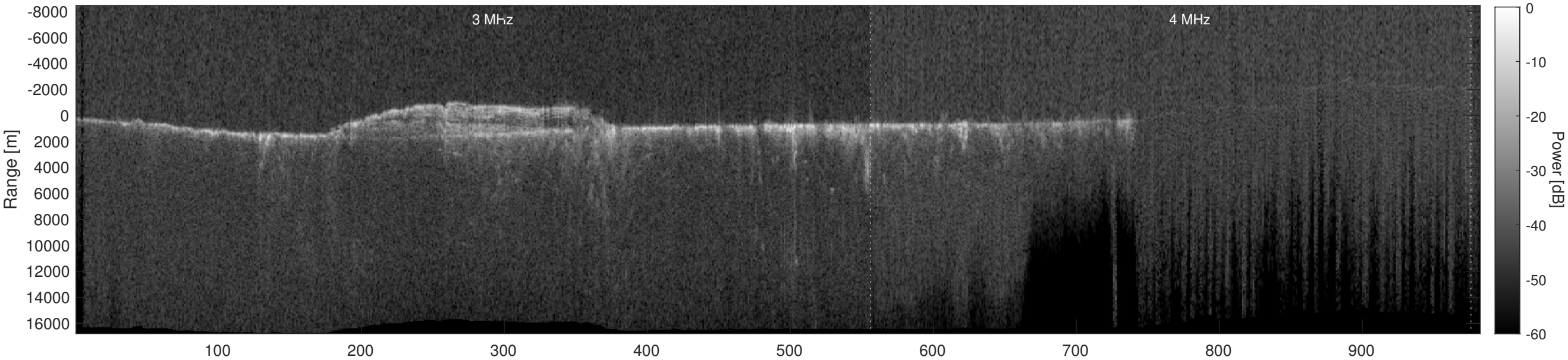
Orbit 13833, Depth-Corrected Cluttergram
