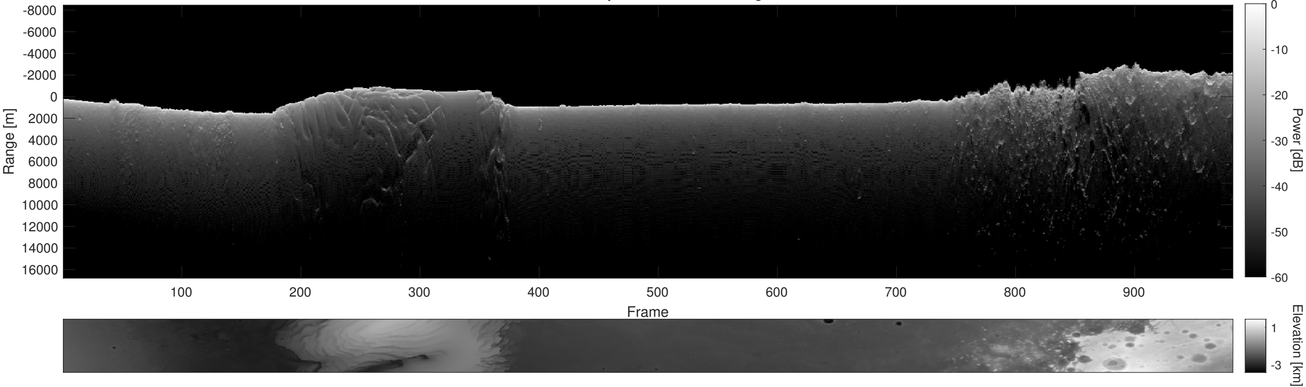
Orbit 13833, Depth-Corrected Cluttergram
