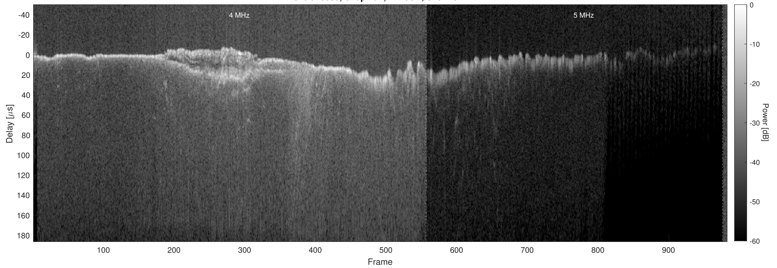
Orbit 13835, Chapman, Window, Channel 2
