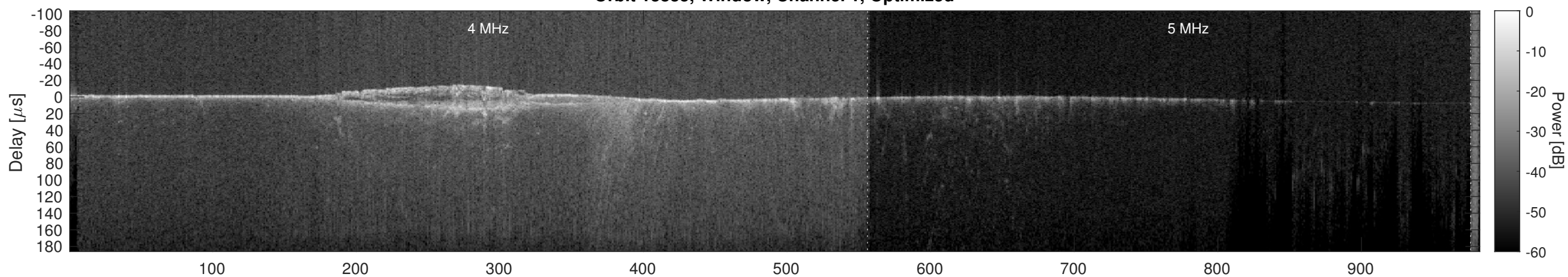
Orbit 13835, Cluttergram
