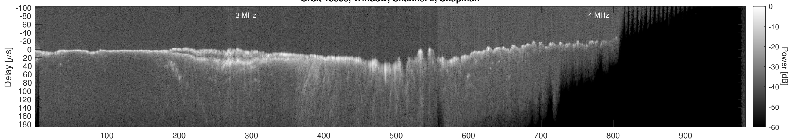
Orbit 13835, Window, Channel 2, Optimized
