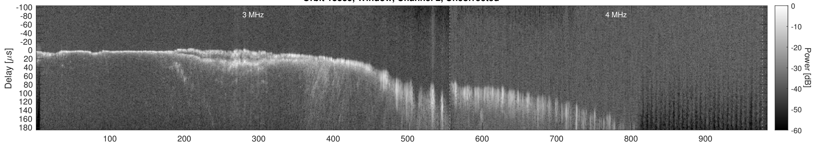
Orbit 13835, Window, Channel 2, Chapman
