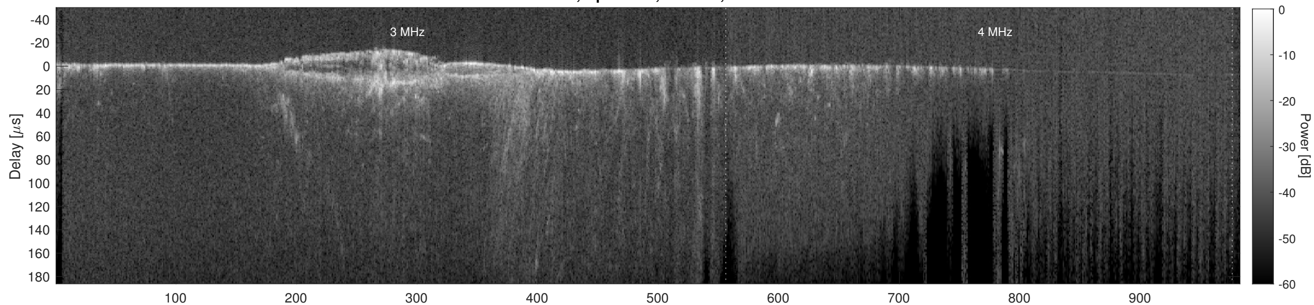
Orbit 13835, Cluttergram
