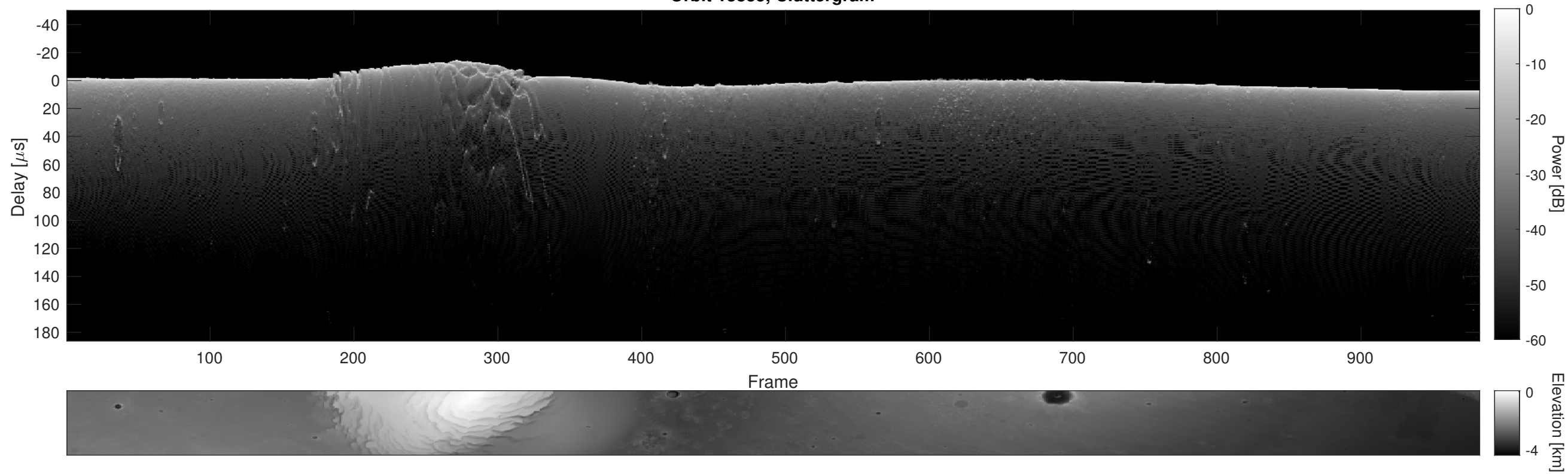
Orbit 13835, Cluttergram
