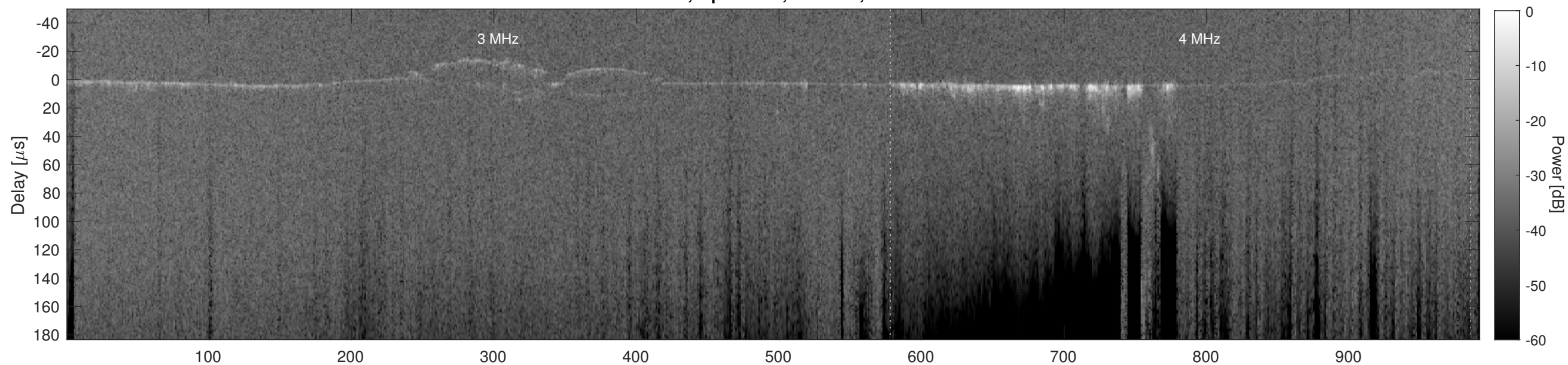
Orbit 13844, Cluttergram
