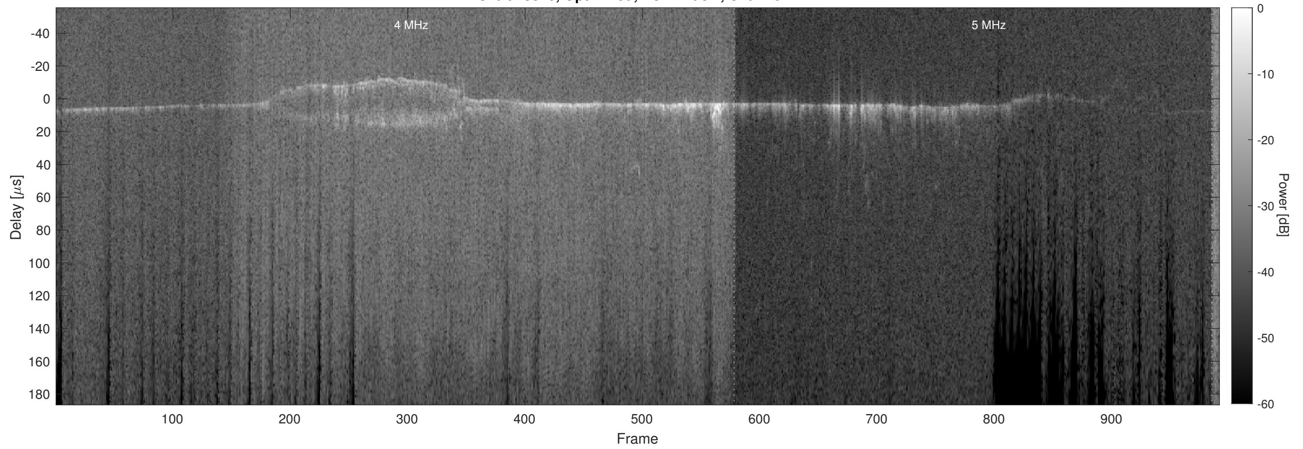
Orbit 13846, Optimized, No Window, Channel 2
