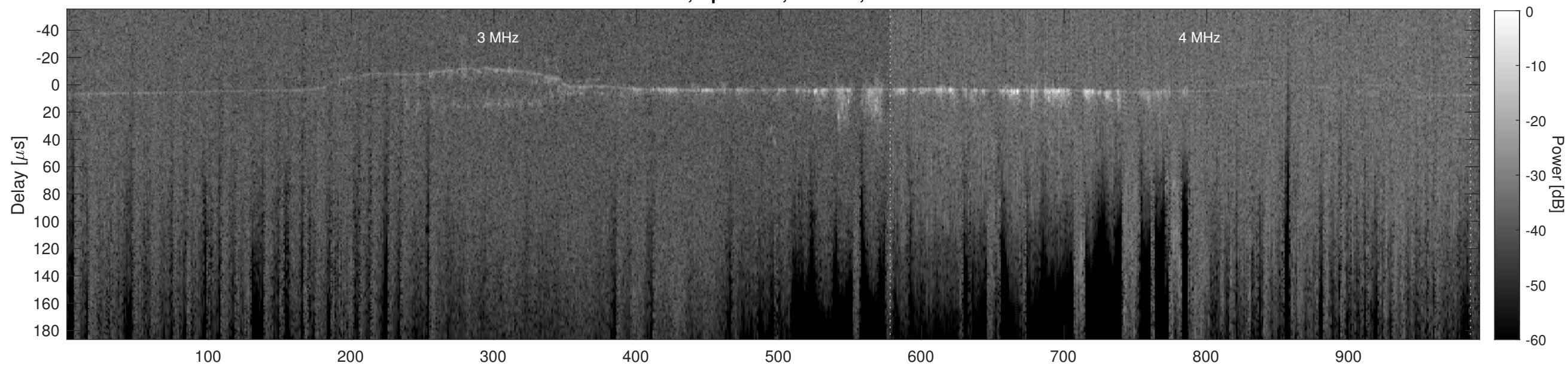
Orbit 13846, Cluttergram
