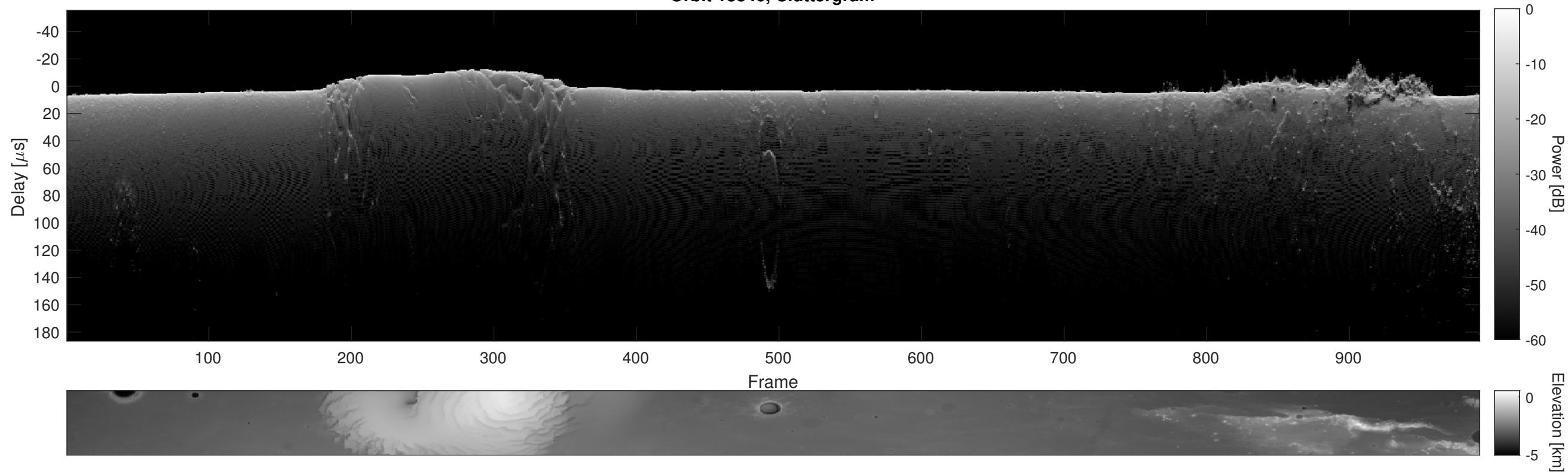
Orbit 13846, Cluttergram
