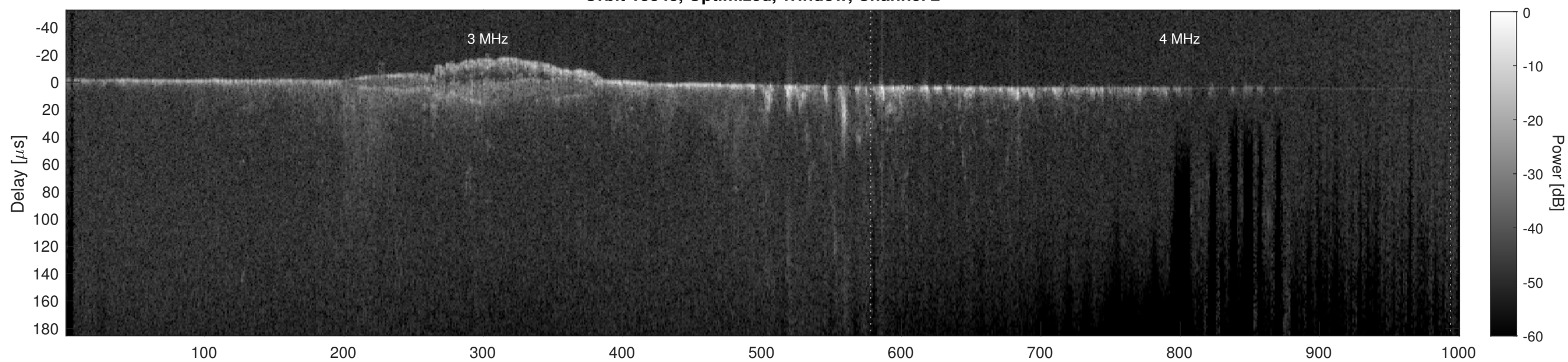
Orbit 13848, Cluttergram
