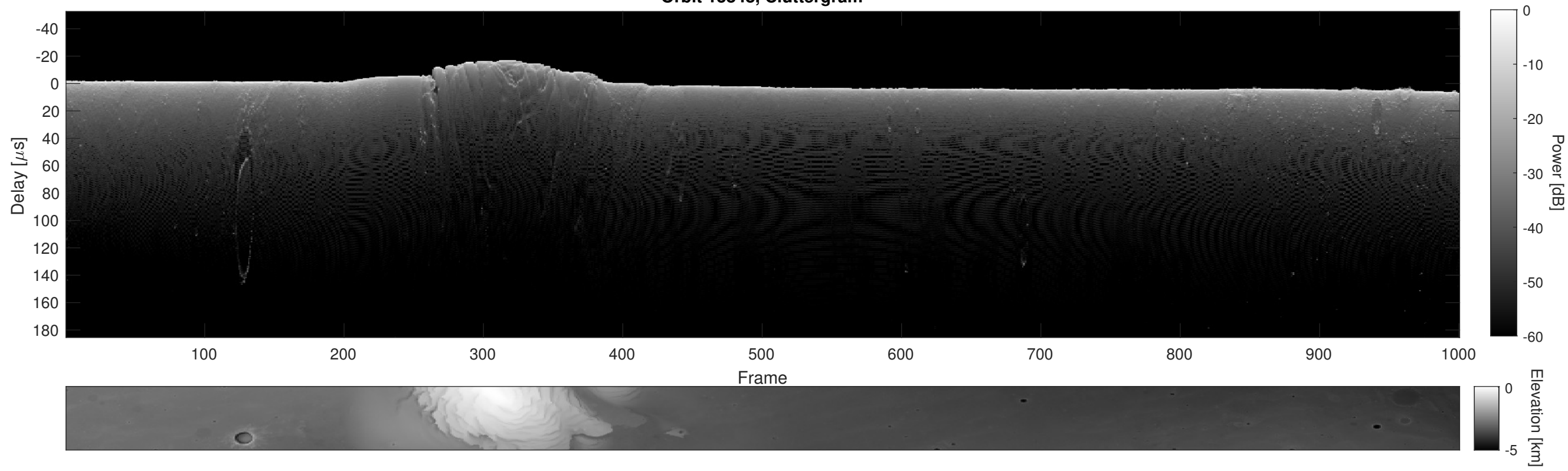
Orbit 13848, Cluttergram
