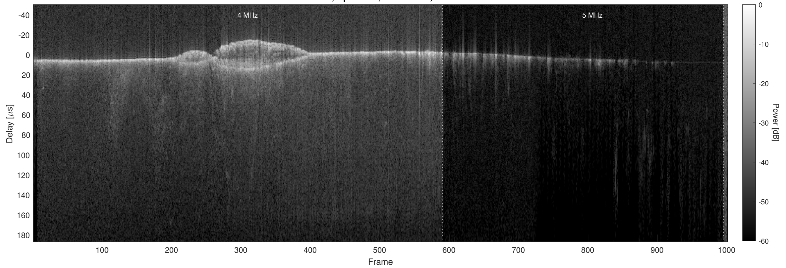
Orbit 13850, Optimized, No Window, Channel 2
