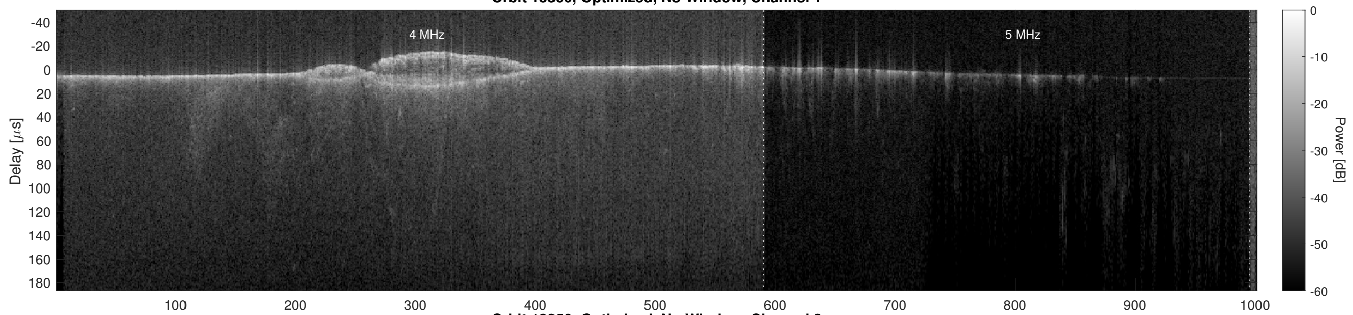
Orbit 13850, Optimized, No Window, Channel 2
