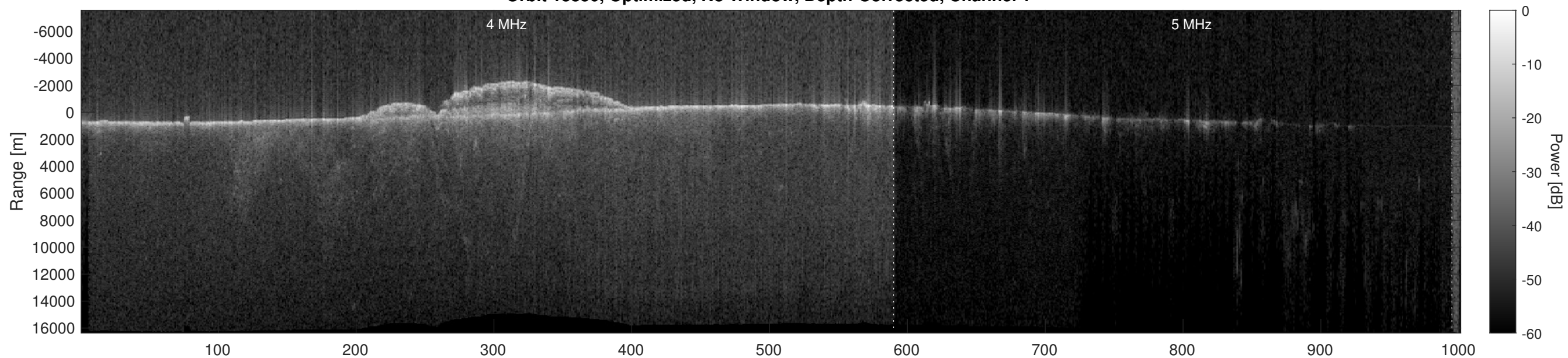
Orbit 13850, Optimized, No Window, Depth-Corrected, Channel 2
