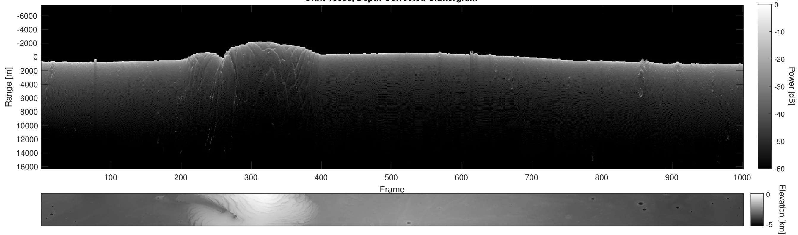
Orbit 13850, Depth-Corrected Cluttergram
