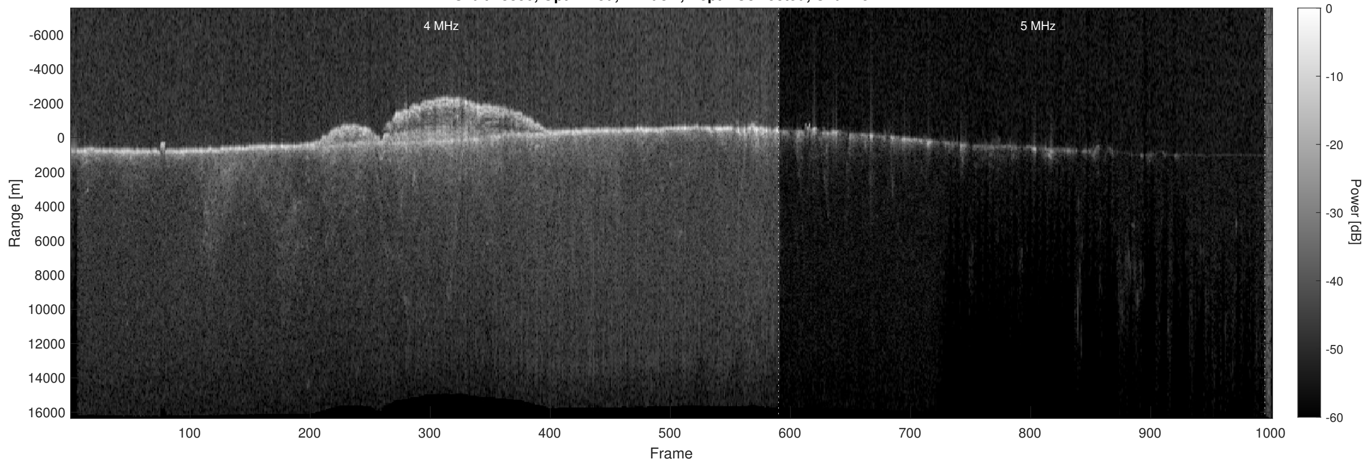
Orbit 13850, Optimized, Window, Depth-Corrected, Channel 2
