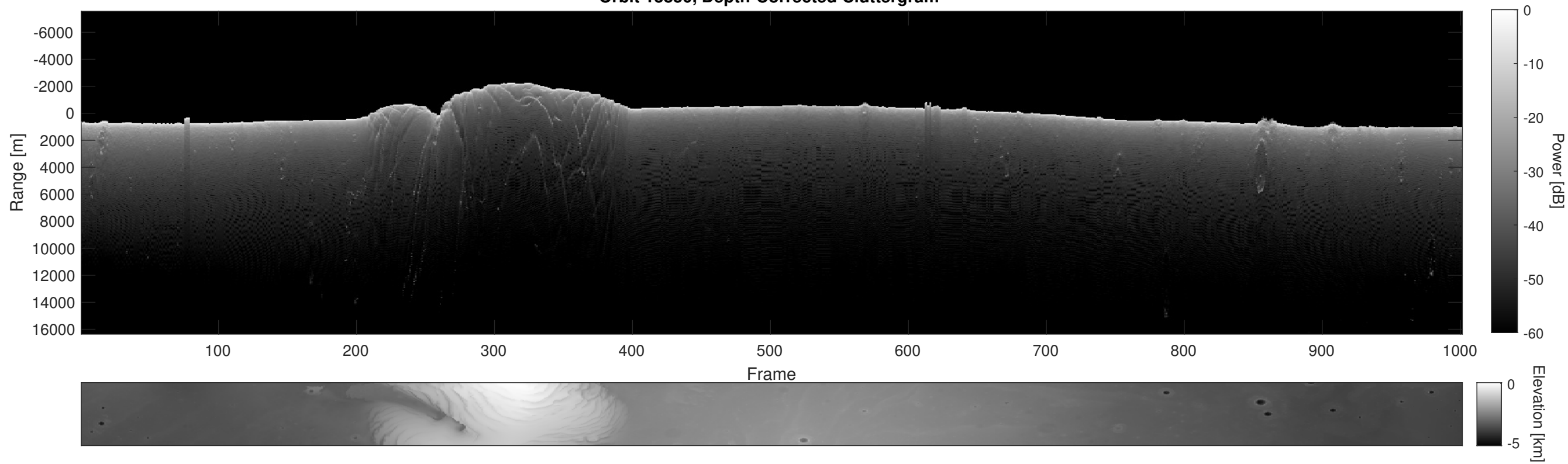
Orbit 13850, Depth-Corrected Cluttergram
