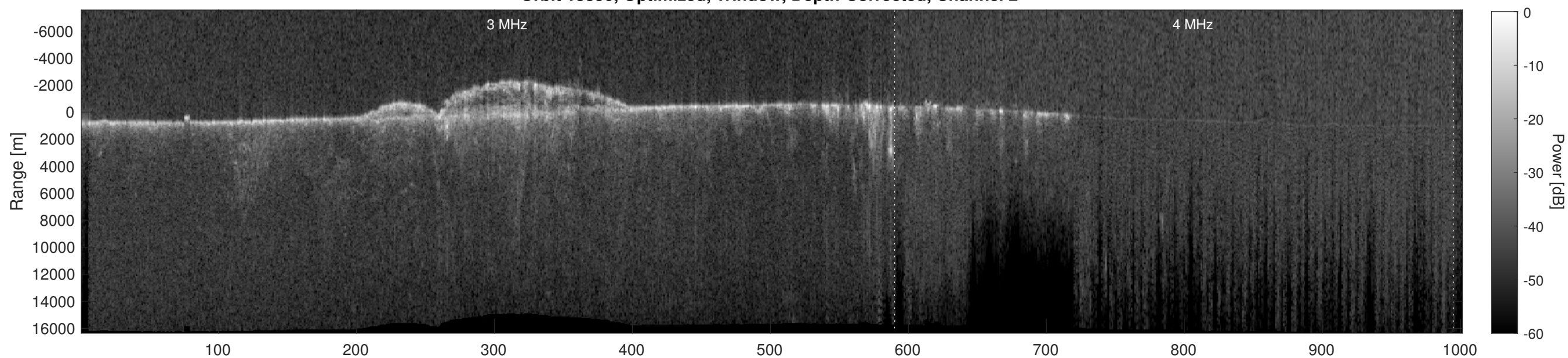
Orbit 13850, Depth-Corrected Cluttergram
