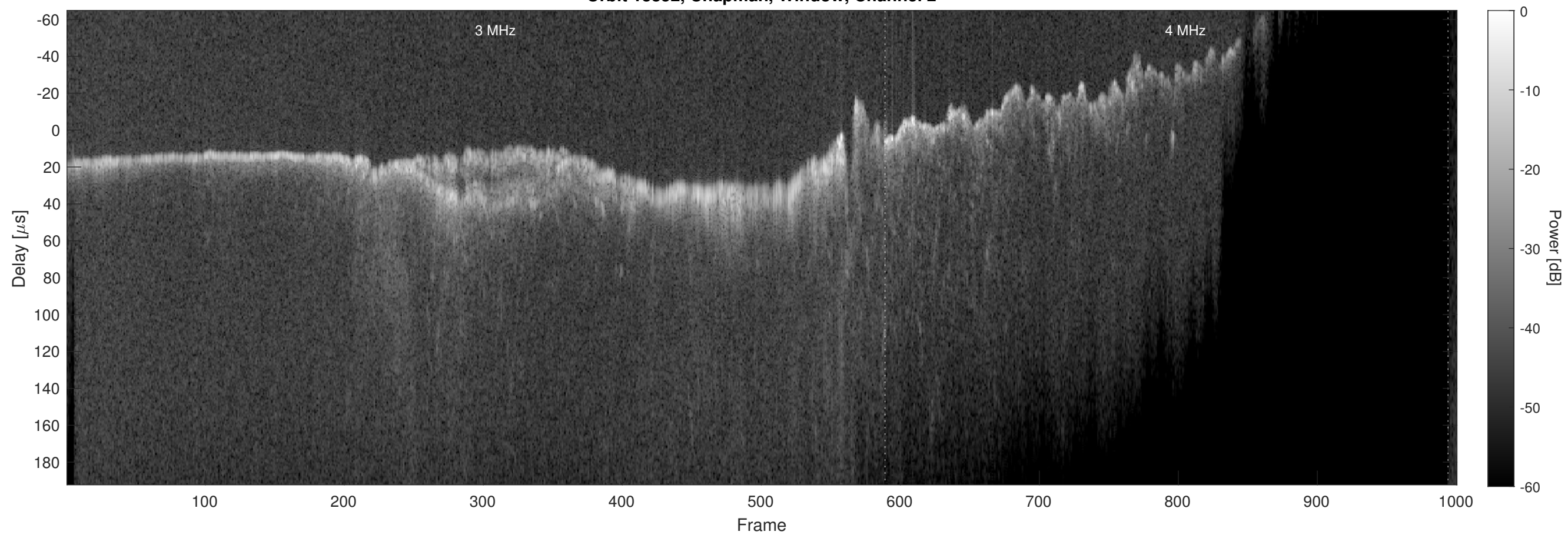
Orbit 13852, Chapman, Window, Channel 2
