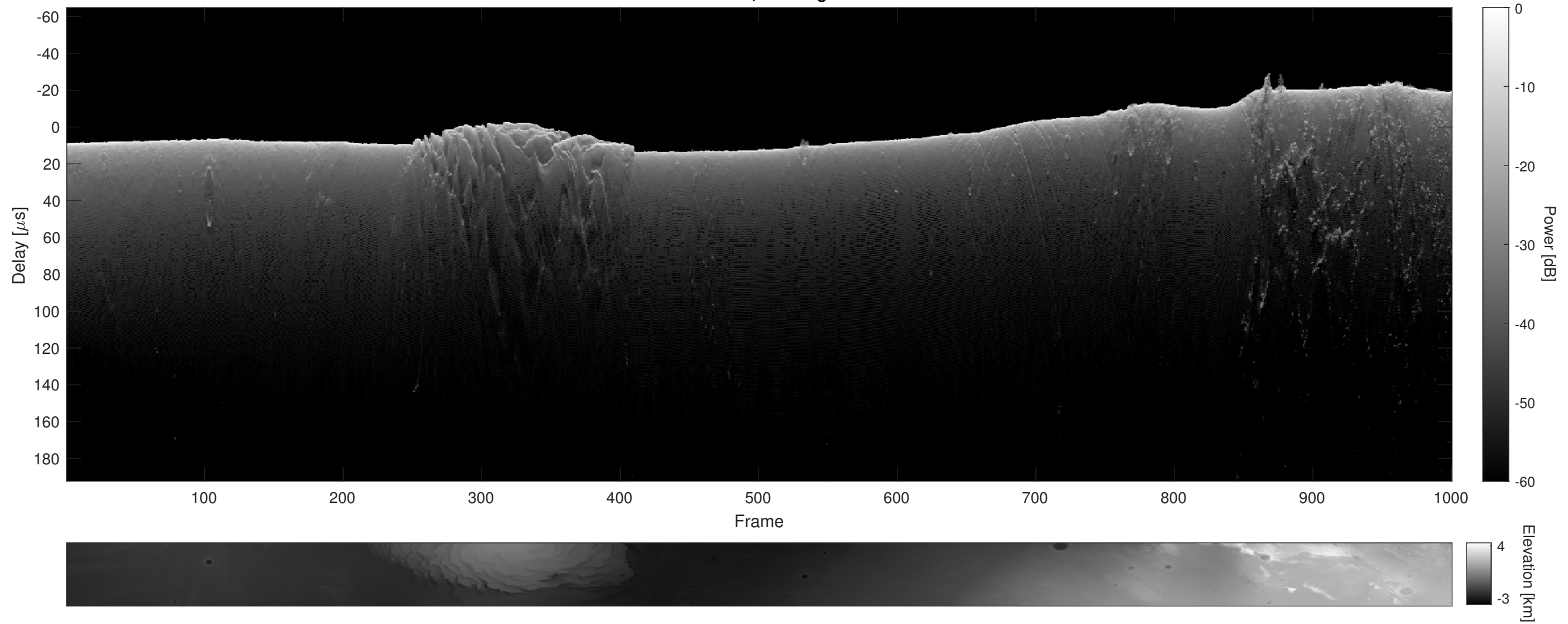
Orbit 13852, Cluttergram
