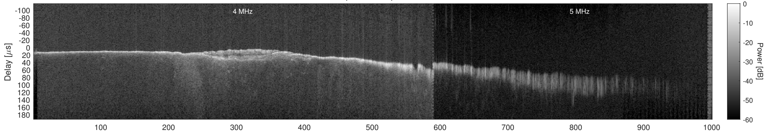
Orbit 13852, Window, Channel 1, Chapman
