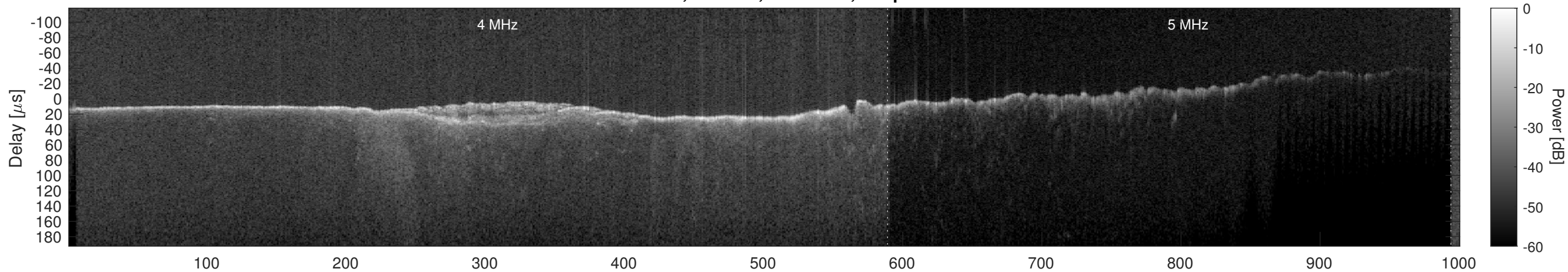
Orbit 13852, Window, Channel 1, Optimized
