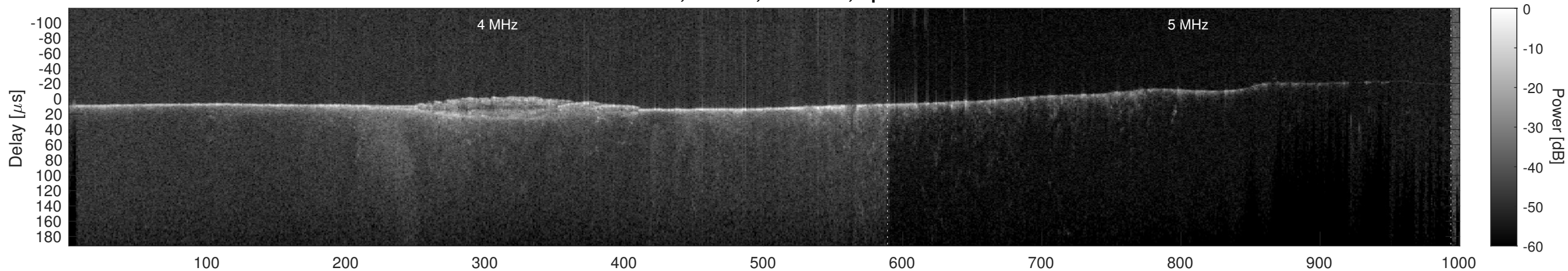
Orbit 13852, Cluttergram
