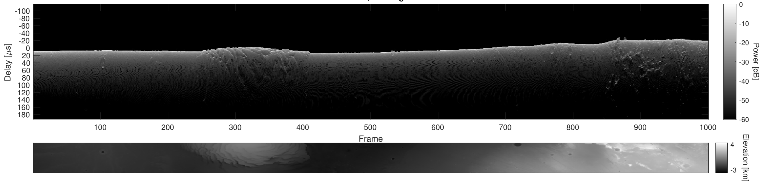
Orbit 13852, Cluttergram
