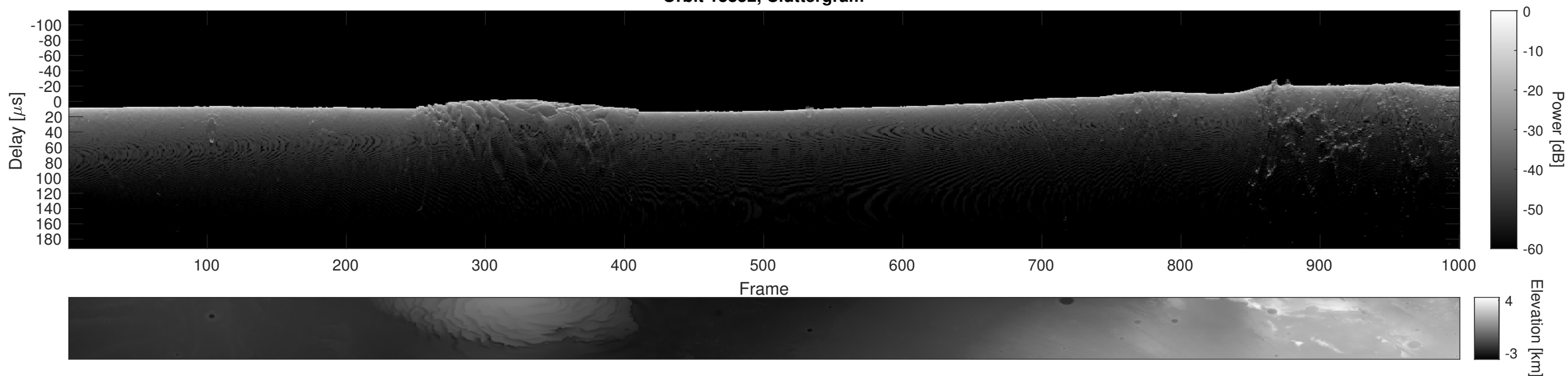
Orbit 13852, Cluttergram
