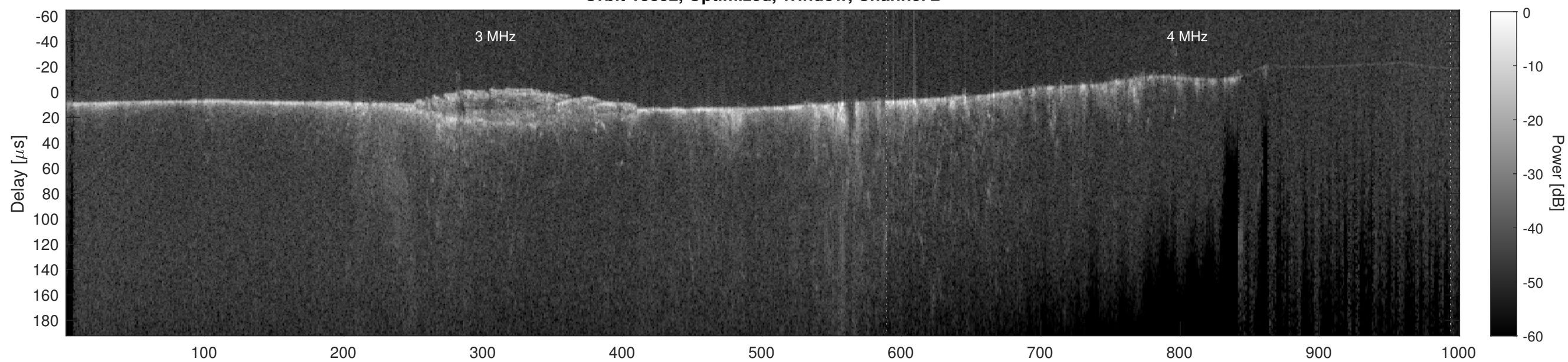
Orbit 13852, Cluttergram
