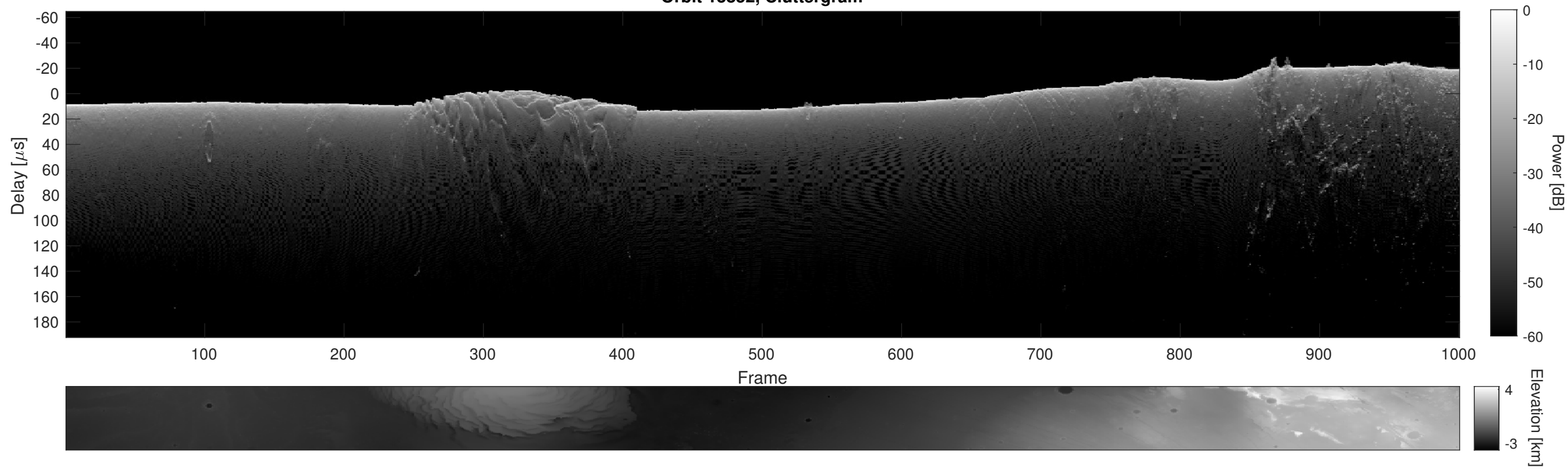
Orbit 13852, Cluttergram
