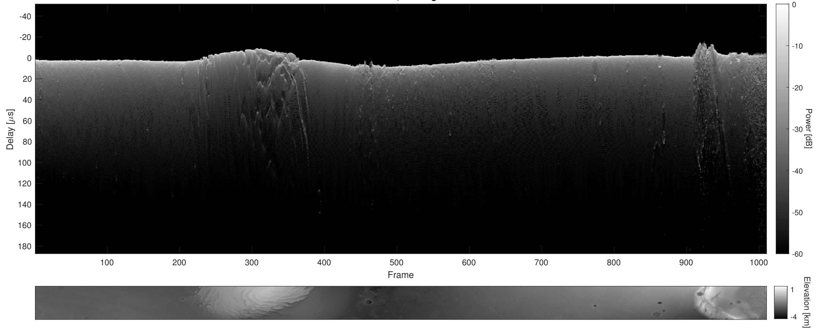
Orbit 13856, Cluttergram
