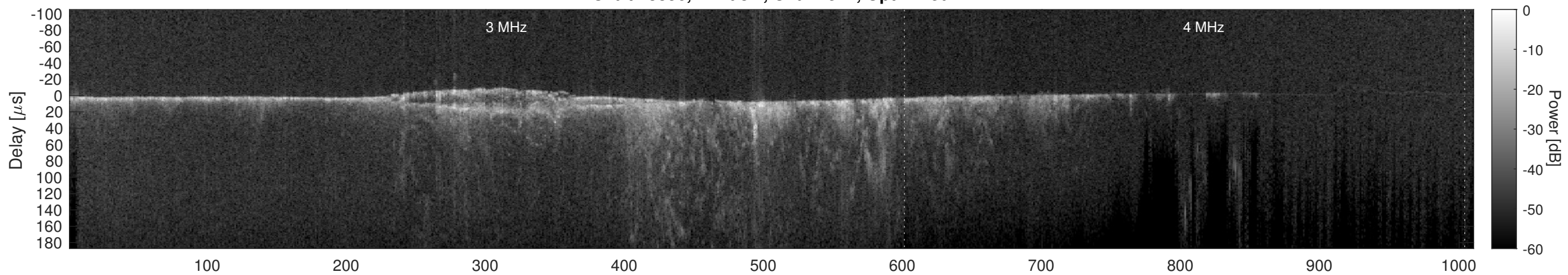
Orbit 13856, Cluttergram
