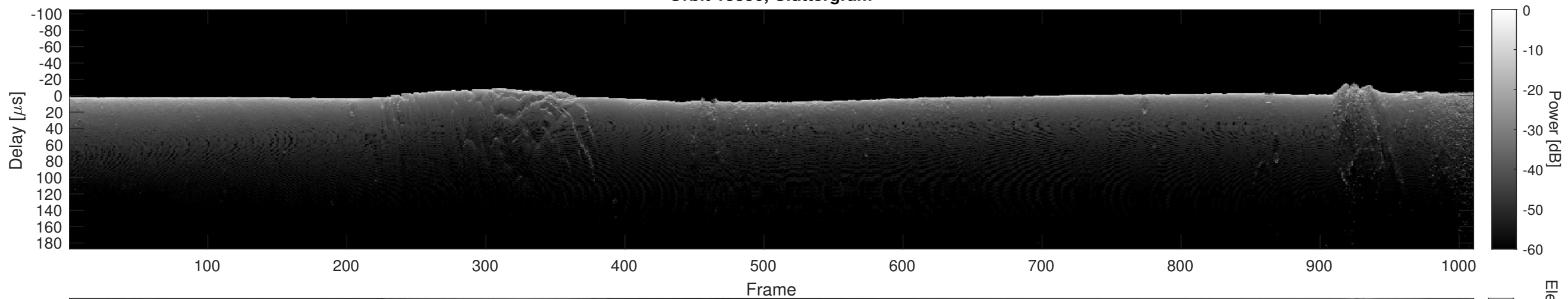
Orbit 13856, Cluttergram
