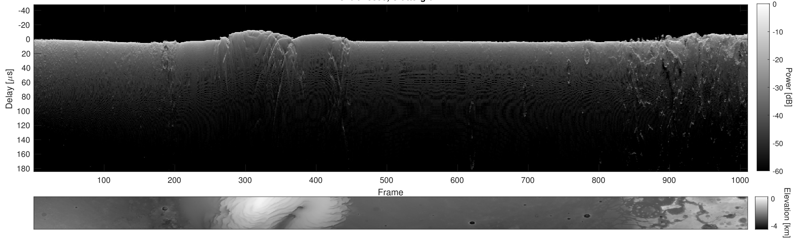
Orbit 13858, Cluttergram
