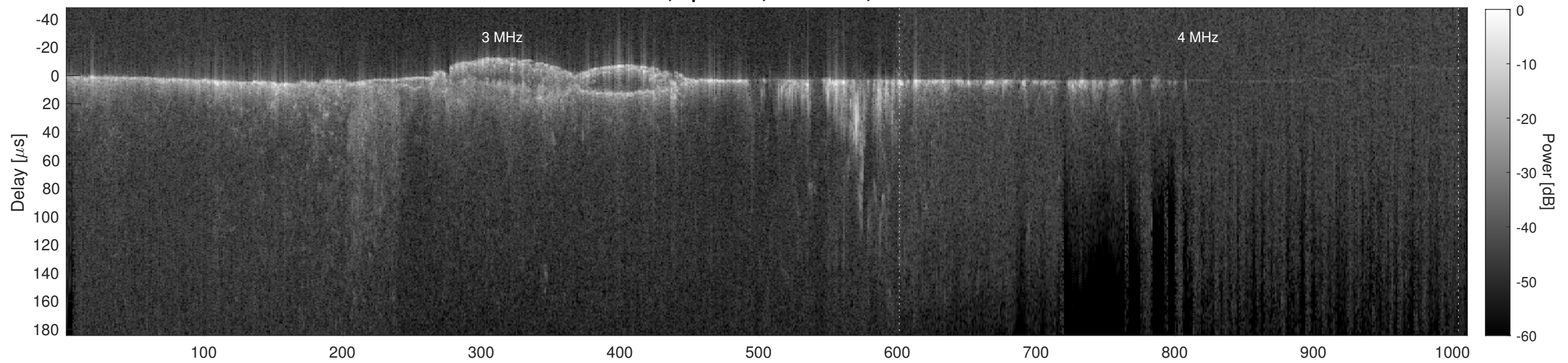
Orbit 13858, Cluttergram
