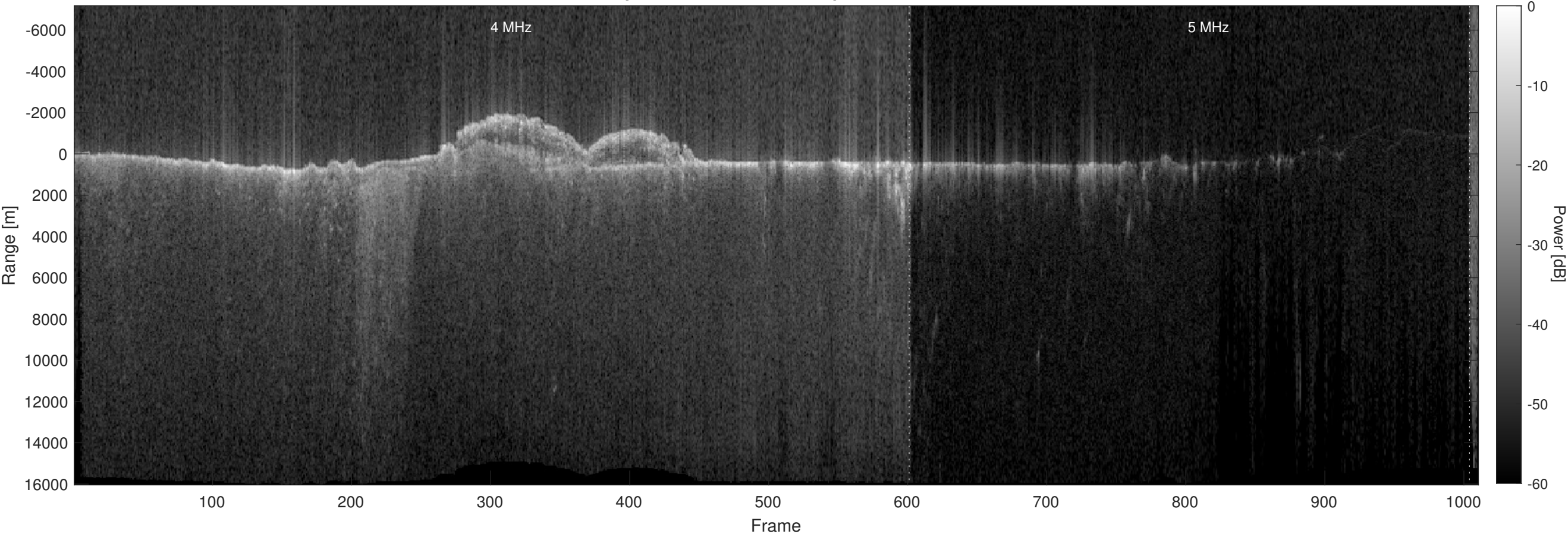
Orbit 13858, Optimized, No Window, Depth-Corrected, Channel 2
