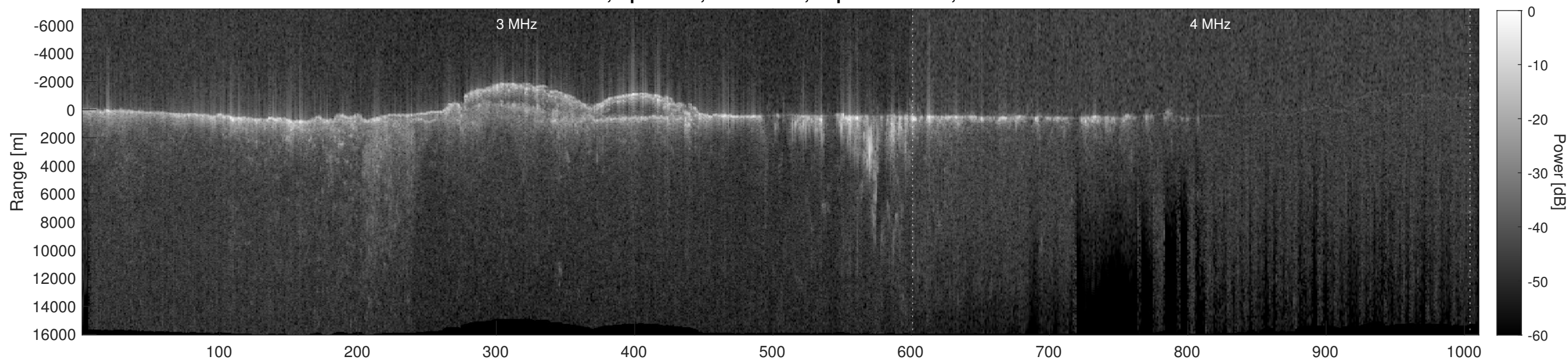
Orbit 13858, Depth-Corrected Cluttergram
