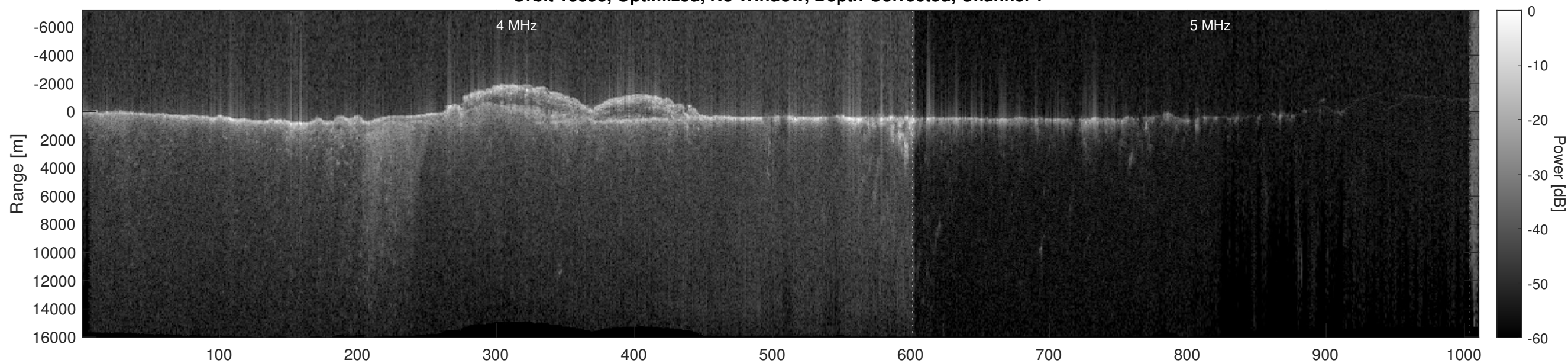
Orbit 13858, Optimized, No Window, Depth-Corrected, Channel 2
