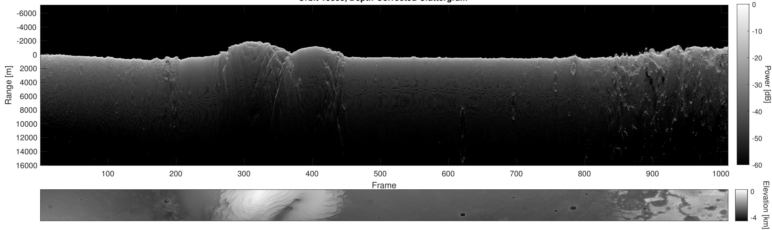
Orbit 13858, Depth-Corrected Cluttergram
