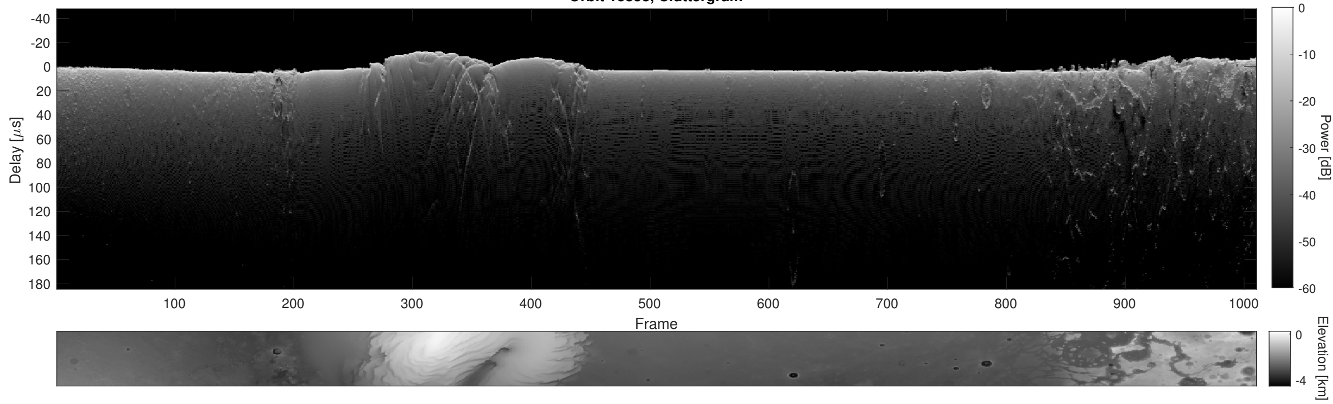
Orbit 13858, Cluttergram
