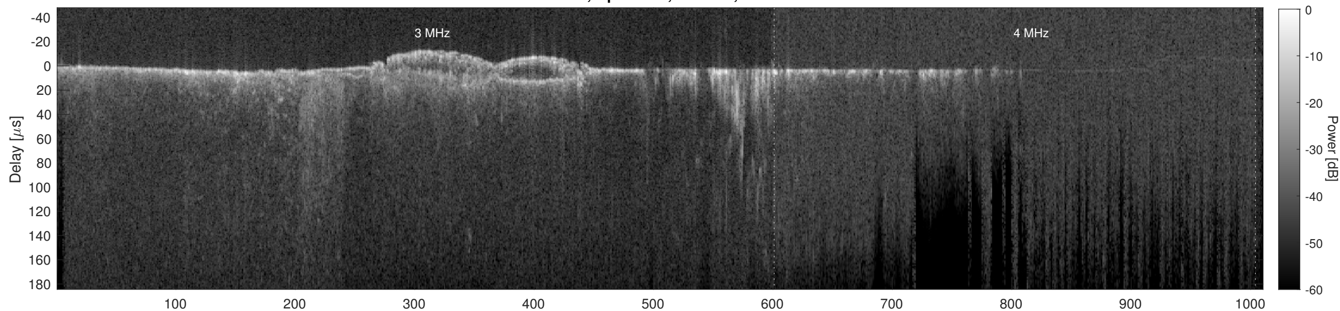
Orbit 13858, Cluttergram
