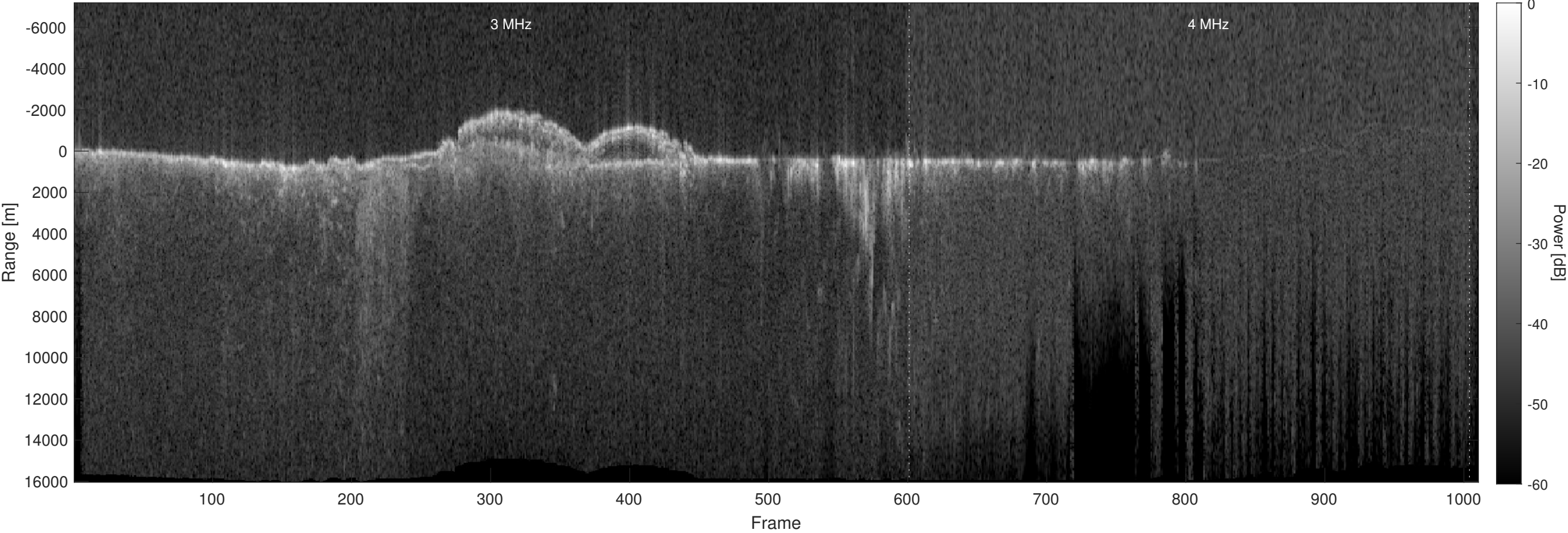
Orbit 13858, Optimized, Window, Depth-Corrected, Channel 2
