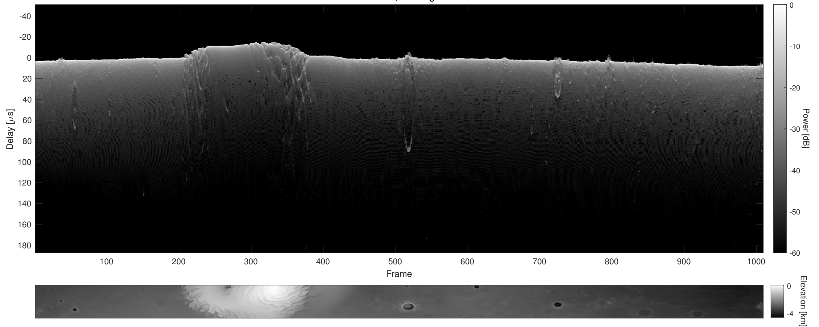
Orbit 13860, Cluttergram
