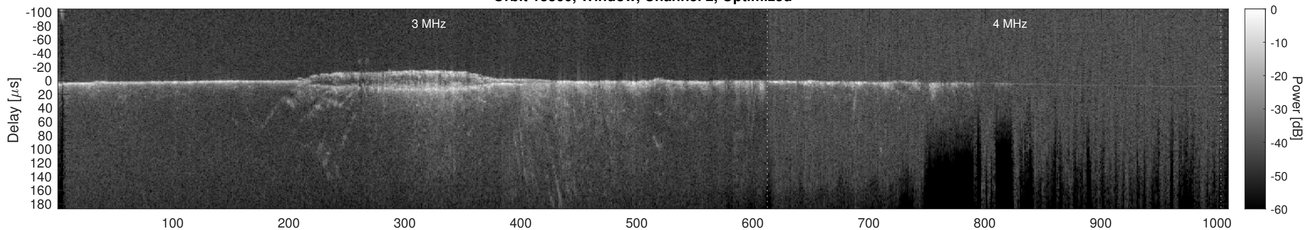
Orbit 13860, Cluttergram
