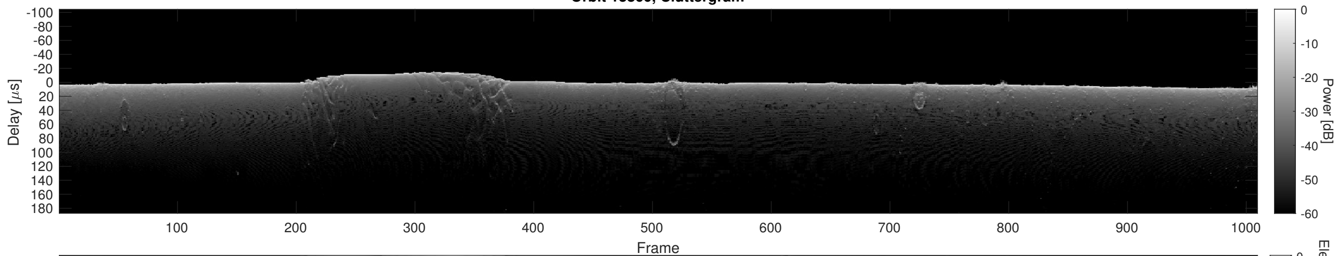
Orbit 13860, Cluttergram
