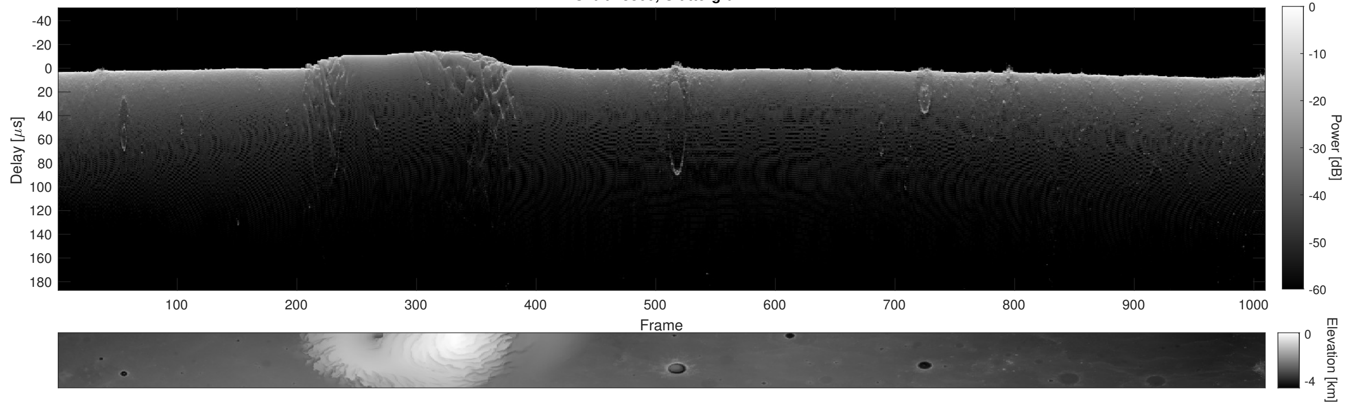
Orbit 13860, Cluttergram
