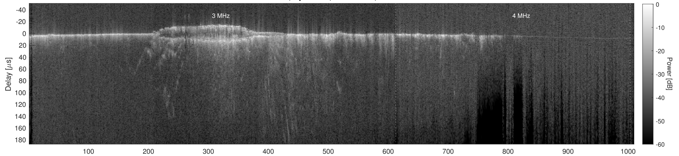
Orbit 13860, Cluttergram
