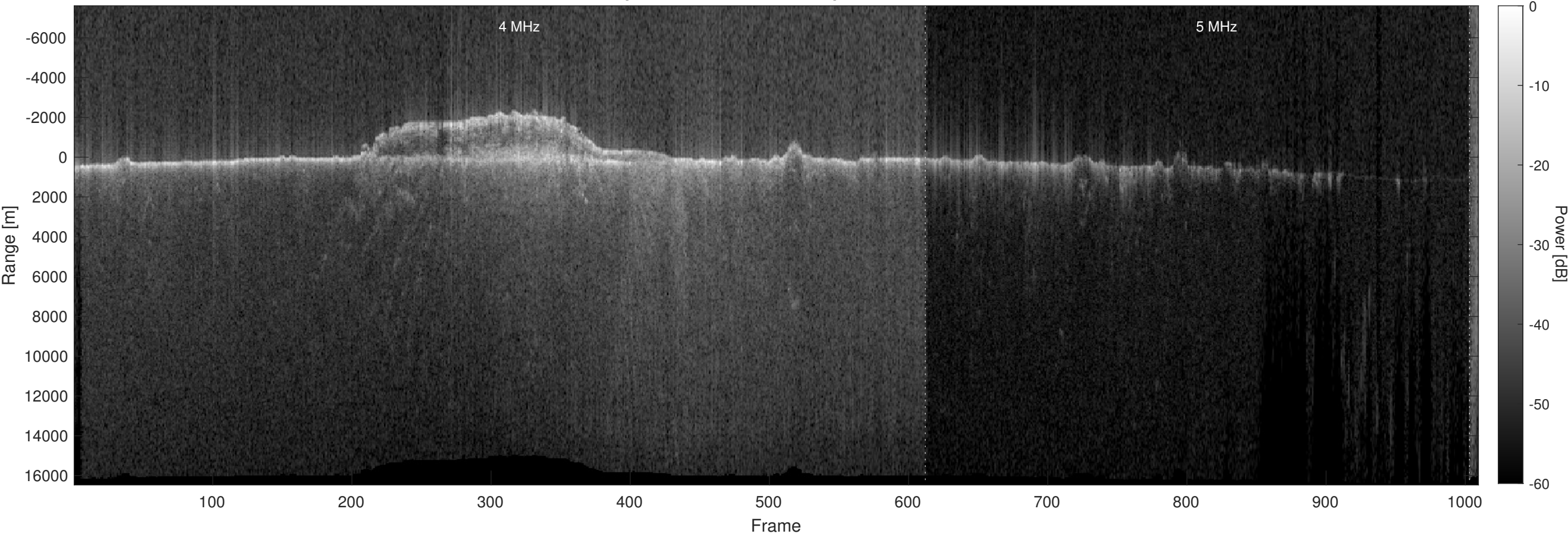
Orbit 13860, Optimized, No Window, Depth-Corrected, Channel 2
