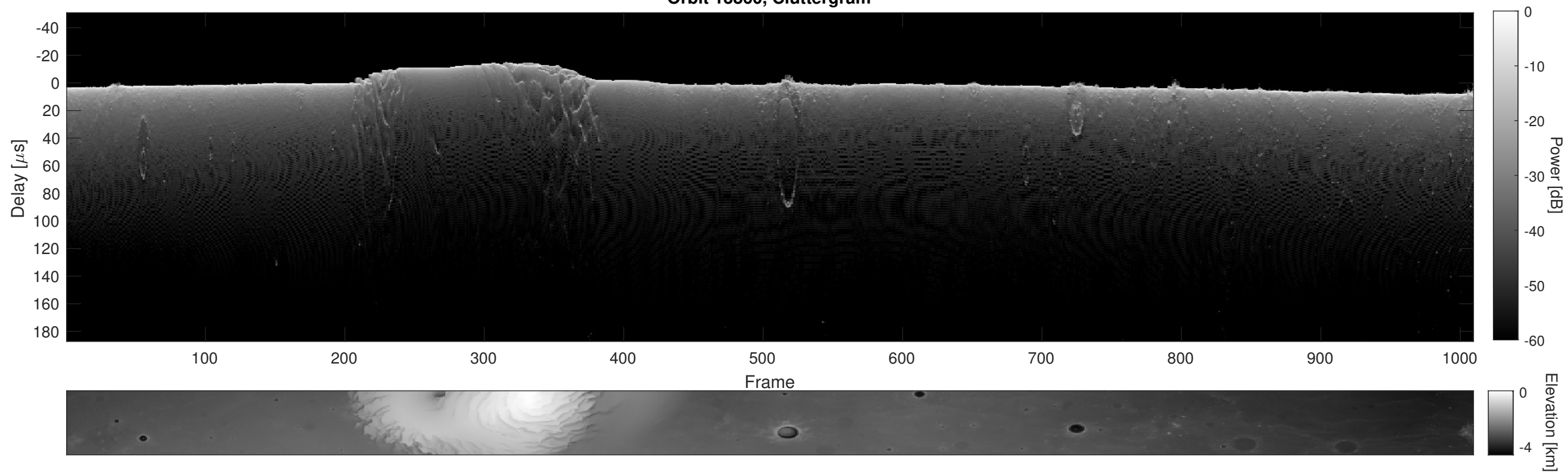
Orbit 13860, Cluttergram
