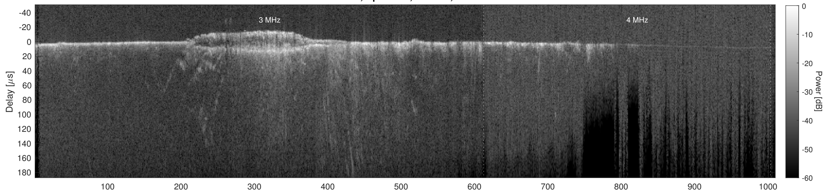
Orbit 13860, Cluttergram
