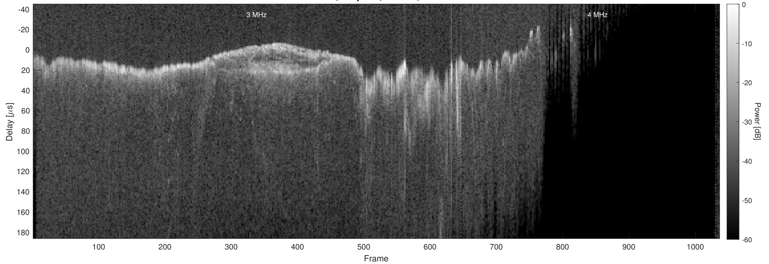
Orbit 13875, Chapman, Window, Channel 2
