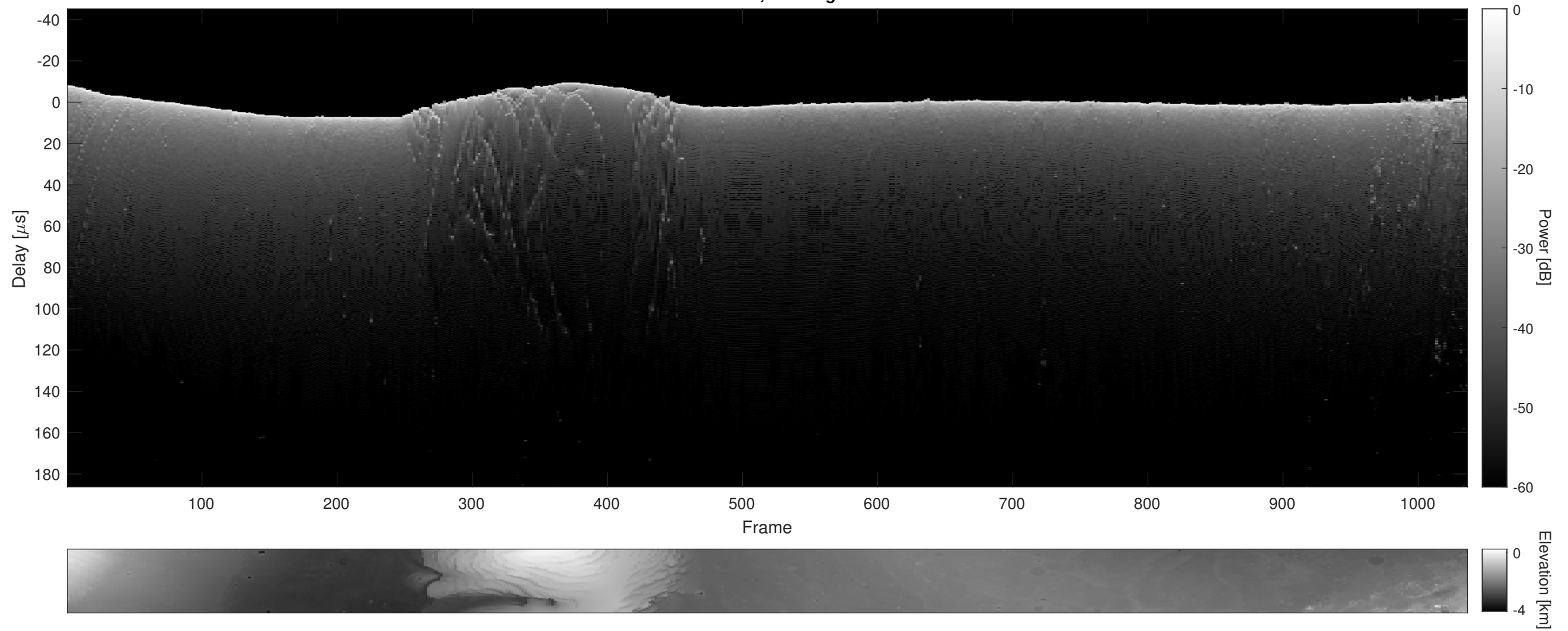
Orbit 13875, Cluttergram
